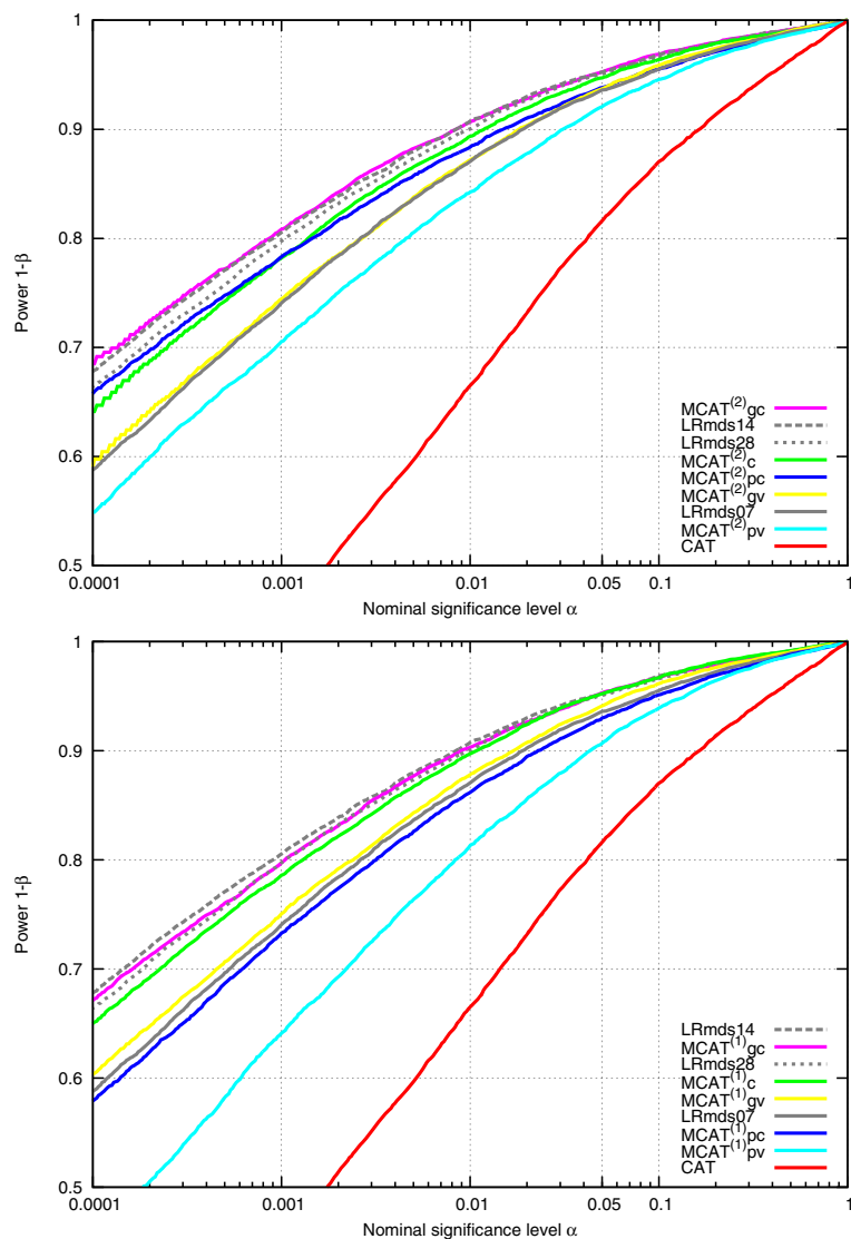
Figure 1 ROC curve. Power simulation of 11,010 SNPs, 1845 individuals. P-values are corrected via genomic control using the corresponding inflation factor from the simulation under H_0 . The abscissas are given in logarithmic scale. The upper plot compares the MCAT (2) with the principal components approach. The lower plot shows the asymptotic test MCAT (1) . The subscripts in the legend denote the employed structures: clusters c , groups (pairs) with cluster validation gc ( pc ) and groups (pairs) with vicinity validation gv ( pv ).
