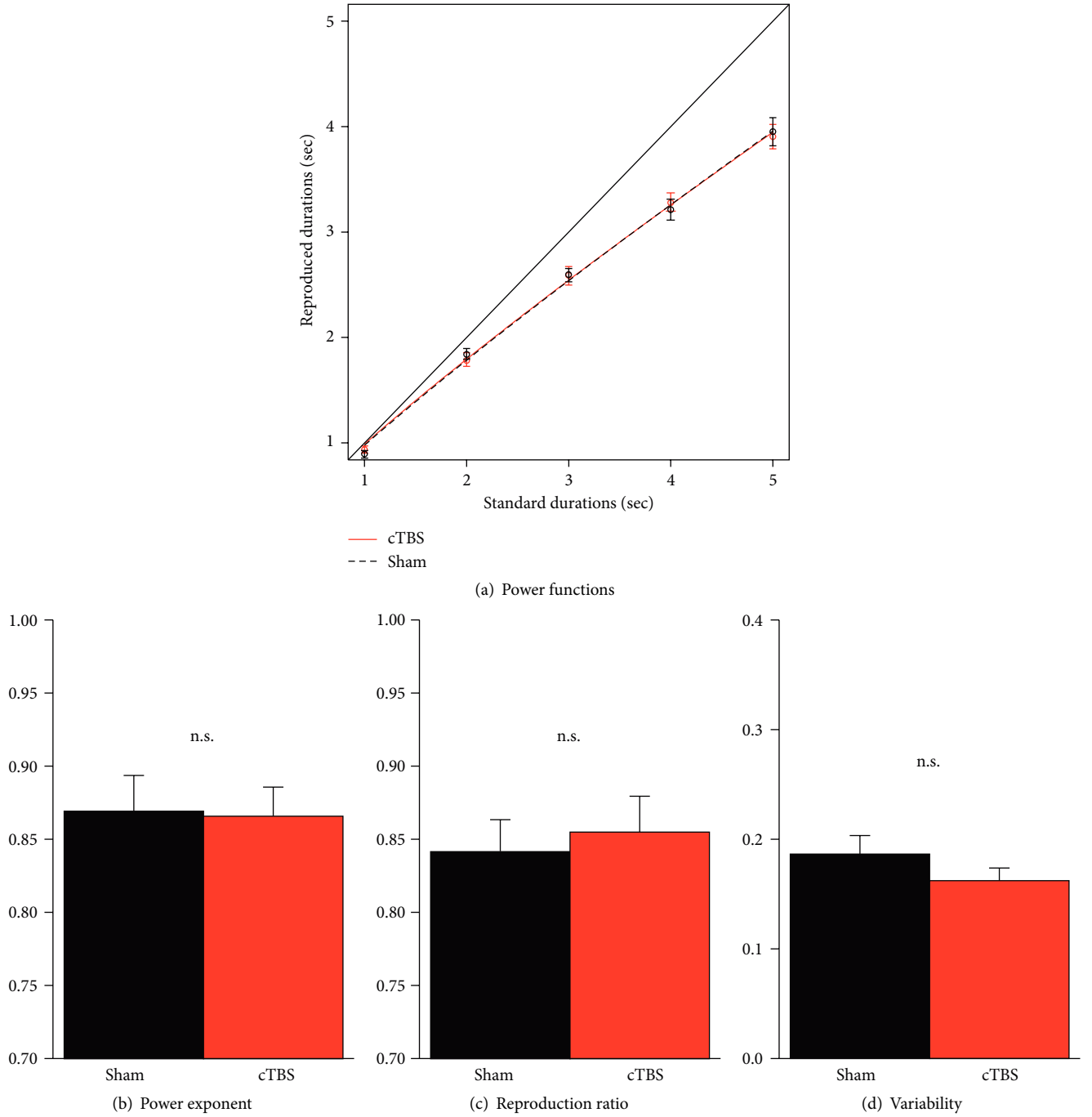
FIGURE 4: (a) Averaged power functions according to the reproduction data. No differences between cTBS (red bars) and sham stimulation (black bars) were found for the power exponent (b), the ratio between reproduced and standard durations, (c) and response variability (d). Error bars show standard errors of the mean across subjects.
