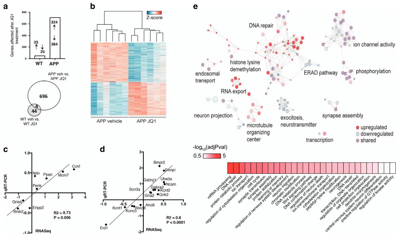
Figure 3. JQ1-induced gene expression in WT and APP mice. (a) Upper panel: number of up- and downregulated genes affected by JQ1 treatment in WT and APP mice. Lower panel: Venn diagram showing limited overlap of genes affected in WT and in APP mice. (b) Heatmap of differentially expressed genes in APP-vehicle vs APP-JQ1 animals showed two main clusters of up- and downregulated genes. (c) qPCR was performed for selected genes affected by JQ1 treatment in WT mice. Correlation analysis shows that qPCR data were able to confirm RNA-seq findings. (d) qRT PCR was performed for selected genes affected by JQ1 treatment in APP mice. Correlation analysis shows that qPCR data were able to confirm RNA-seq findings. (e) Network of functional categories represented by JQ1-associated changes in APP animals based on the Biological Process ontology. The size of the nodes correlates inversely with statistical significance. Categories of upregulated genes are red, downregulated genes are blue and those where there are both up- and downregulation are purple.
