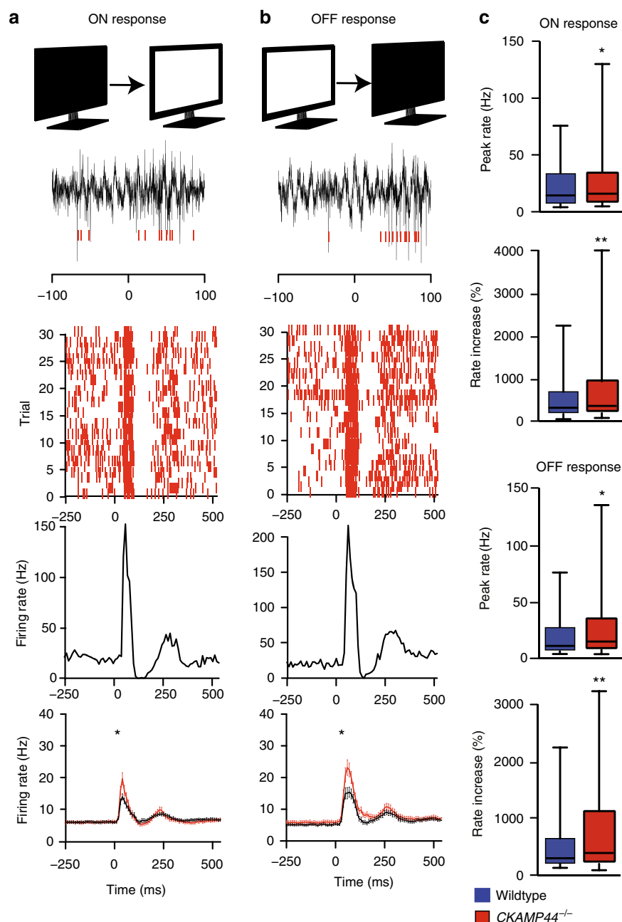
Fig. 5 CKAMP44 decreases peak firing rate of ON and OFF-responses in vivo. a ON-response amplitude is significantly higher in CKAMP44 -/- than in wildtype mice. ON-responses were observed briefly after increasing the light intensity of the monitor ( n = 542 dLGN neurons in 6 wildtype and 430 dLGN neurons in 6 CKAMP44 -/- mice; mean \pm SEM). b Deletion of CKAMP44 increases also the OFF-response amplitude (mean \pm SEM, Mann-Whitney test) ( n = 309 dLGN neurons in 6 wildtype and 285 dLGN neurons in 6 CKAMP44 -/- mice). a, b Raw traces of tetrode recordings are shown on the top, raster and peristimulus time histograms in the middle and average ON- and OFF-responses at the bottom. Red bars indicate spikes of dLGN neurons. c Quantification of the peak firing rate and the rate increase for ON- and OFF-responses (box-and-whisker plots showing the median, IQR and 5–95% range, Mann-Whitney test). * p < 0.05 , ** p < 0.01 , *** p < 0.001
