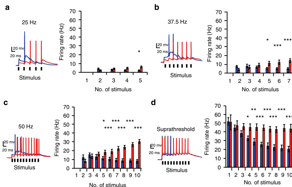
Fig. 4 The influence of CKAMP44 on firing rate increases with optic tract stimulation number and frequency. a–c The difference in firing rates of relay neurons between genotypes increases with stimulation frequency and with the number of stimuli in the train. The optic tract was stimulated with 25 Hz ( a , wildtype: n = 50 , CKAMP44 -/- : n = 67 ), 37.5 Hz ( b , wildtype: n = 49 , CKAMP44 -/- : n = 28 ), and 50 Hz ( c , wildtype: n = 45 , CKAMP44 -/- : n = 55 ) and firing rates for different stimulus numbers were calculated by dividing the cumulative action potential number by the respective stimulation duration (mean \pm SEM, Mann–Whitney test). d Firing rates are significantly higher in relay neurons of CKAMP44 -/- mice than in those of wildtype mice when stimulating such that the first stimulus was just suprathreshold and elicited an action potential (wildtype: n = 31 , CKAMP44 -/- : n = 11 , mean \pm SEM; responses to 3, 4, and 5 stimuli: Mann–Whitney test, other responses: t -test). * p < 0.05 , ** p < 0.01 , *** p < 0.001
