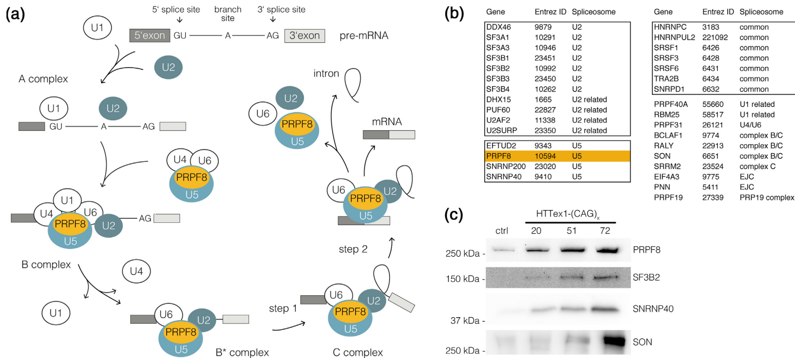
Fig. 1. Proteins that aberrantly bind mutant HTTex1 RNA are associated with splicing. (a) Schematic showing the splicing cycle. PRPF8, a U5-subunit, is indicated in yellow. (b) HTT RNA-binding proteins were identified by RNA–protein pull-down followed by mass spectrometry. Mutant HTT RNA-interacting proteins (36 proteins binding in a length-dependent manner) are significantly enriched for splicing factors (see also Supplementary Figs. 1, 2, 3, and Supplementary Table 1). A list of these proteins is shown. (c) RNA–protein pull-downs of HTTex1 RNA with different repeat lengths analyzed on Western blot detecting the splice factors PRPF8, SF3B2, SNRNP40 and SON. PRPF8 and SNRNP40 are components of the U5 snRNP, SF3B3 is a component of the U2 snRNP. SON probably acts by facilitating the interaction between SRSF2 and the RNA polymerase II, which is required for formation of the earliest ATP-dependent splicing complex and for interactions of U1 and U2 snRNPs with pre-mRNA.
