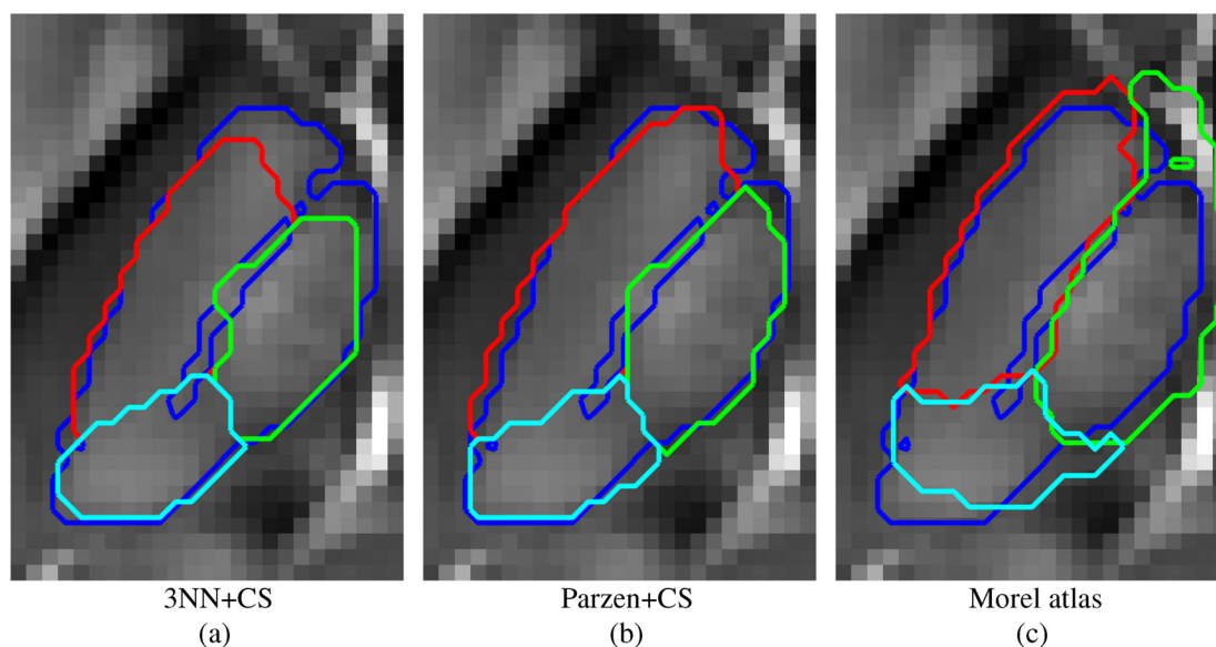
FIGURE 6 Convex segmentation results (for the template Dataset II) from different algorithmic implementations and the Morel atlas overlay onto the Dataset II QSM template. The blue overlay represents the ground truth's outer contour. Red, green and cyan contours are the results for the different approaches
