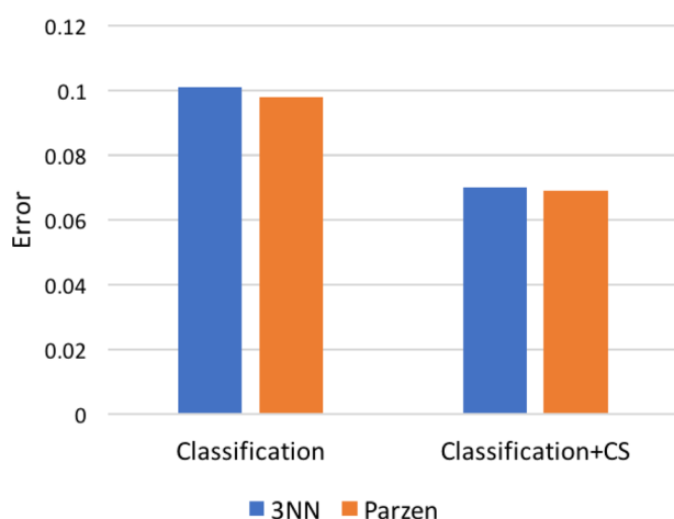
FIGURE 5 Error rates for (left) classification and (right) classification followed by convex segmentation (CS) on Dataset II average template data. Bars represent misclassification frequency, that is, overall proportion of errors relative to the manually traced ground truth
