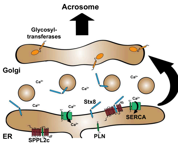
Fig. 3 The role of SPPL2c in the murine testis. SPPL2c shows selective expression in elongated spermatids. In these cells, SPPL2c resides in the endoplasmic reticulum (ER). Two in vivo substrates of this protease have been identified: the SNARE protein syntaxin 8 (Stx8) and Phospholamban (PLN), an interactor and inhibitor of the SERCA \text{Ca}^{2+} ATPase. Both proteins accumulate in the testis of SPPL2c-deficient mice. As functional consequences of SPPL2c-deficiency, handling of \text{Ca}^{2+} and membrane trafficking in the secretory pathway are altered in spermatids. SPPL2c -/- spermatids show a reduced cytoplasmic \text{Ca}^{2+} concentration. Furthermore, the organisation of the Golgi apparatus is less compact which may have implications for the protein delivery to the forming acrosome. Mature SPPL2c -/- sperm cells show an altered glycosylation pattern presumably reflecting alterations of glycosyltransferase trafficking which has been characterised in SPPL2c-overexpressing HEK cells
