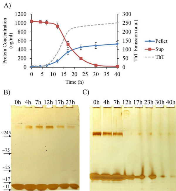
Fig. 5. Studying the different species of aggregates during the \alpha SN fibrillization process. A) BCA protein concentration analysis for soluble (red) and insoluble (blue) fractions during the fibrillization process. ThT is shown as a gray dashed line. Measurement was done at room temperature, pH 7.4. B) Gradient SDS-PAGE (4–16%) analysis of samples from different incubation times during the fibrillization process. Monomers were observed below the 17 kD band and oligomers were observed above the 245 kD band of protein ladder. C) Gradient native-PAGE (4–16%) analysis of samples from different incubation times during the fibrillization process. Gels were developed using the silver staining method.
