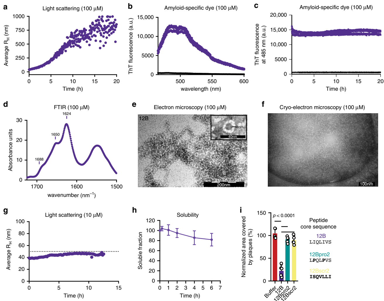
Fig. 2 Peptide 12B organizes into amyloid-like structures in vitro. a Hydrodynamic radius ( R_H ) calculated from the regularization fit of DLS data of peptide 12B (100 \mu M) maturation over time. b Th-T emission spectrum after excitation at 440 nm of buffer (black line) or peptide 12B (100 \mu M, purple line) 5 min after solubilization ( n = 3 independent experiments). c Th-T emission signal of buffer (black line) or peptide 12B (100 \mu M, purple line) at 485 nm after excitation at 440 nm as a function of time. Data represent three independent repeats ( n = 3 independent experiments). d FTIR spectrum of 100 \mu M peptide 12B 5 min after solubilization. TEM ( e ) and cryo-TEM ( f ) of 100 \mu M freshly dissolved peptide 12B (both are one representative image of three independent experiments). g Hydrodynamic radius ( R_H ) calculated from the regularization fit of DLS data of peptide 12B (10 \mu M) maturation over time (dashed line = 50 nm). h Soluble fraction of peptide 12B (10 \mu M) determined after ultracentrifugation (250,000 \times g for 30 min), measured over time, and mean \pm SD is shown ( n = 3 independent experiments). i Quantification of the area covered by plaques of MDCK cells treated with 10 \mu M peptide in a plaque-size reduction assay with influenza A/PR8. Data are normalized to medium-treated cells and the mean \pm SD is shown ( n = 5 independent experiments, statistics: one-way ANOVA with multiple comparison).
