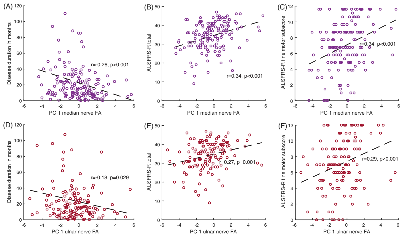
FIGURE 3 Correlations of PC1 with disease durationALS Functional Rating Scale—Revised (ALSFRS-R) total score, and its fine motor subscore. The contrast-driven PC1 for the median (top row) and ulnar nerve (bottom row) sites display significant correlations with disease duration (A, D), ALSFRS-R total score (B, E), and its fine motor subscore (C, F). The positive correlations indicate that patients with better-preserved echoic contrasts tended to score higher on ALSFRS-R scores. The negative correlations with disease duration indicate that the values for PC1 decrease as echoic contrasts decrease over the course of the disease. The relation between PC1 for the median nerve (A) and disease duration reached significance after Bonferroni adjustment, whereas significance did not survive the adjustment for the ulnar nerve (D) [Color figure can be viewed at wileyonlinelibrary.com ]
