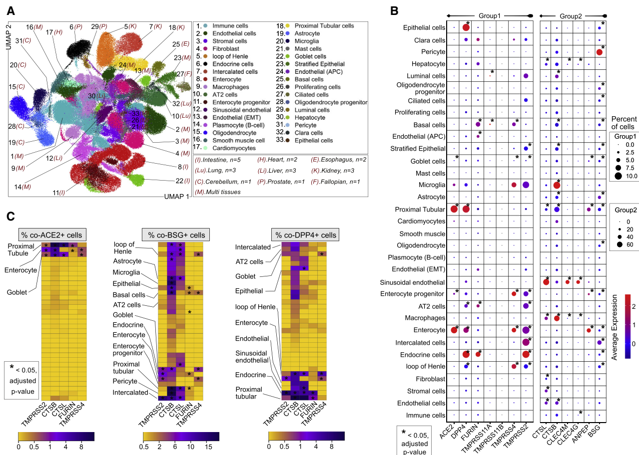
Figure 4. SCARF Expression across 14 Adult Tissues
