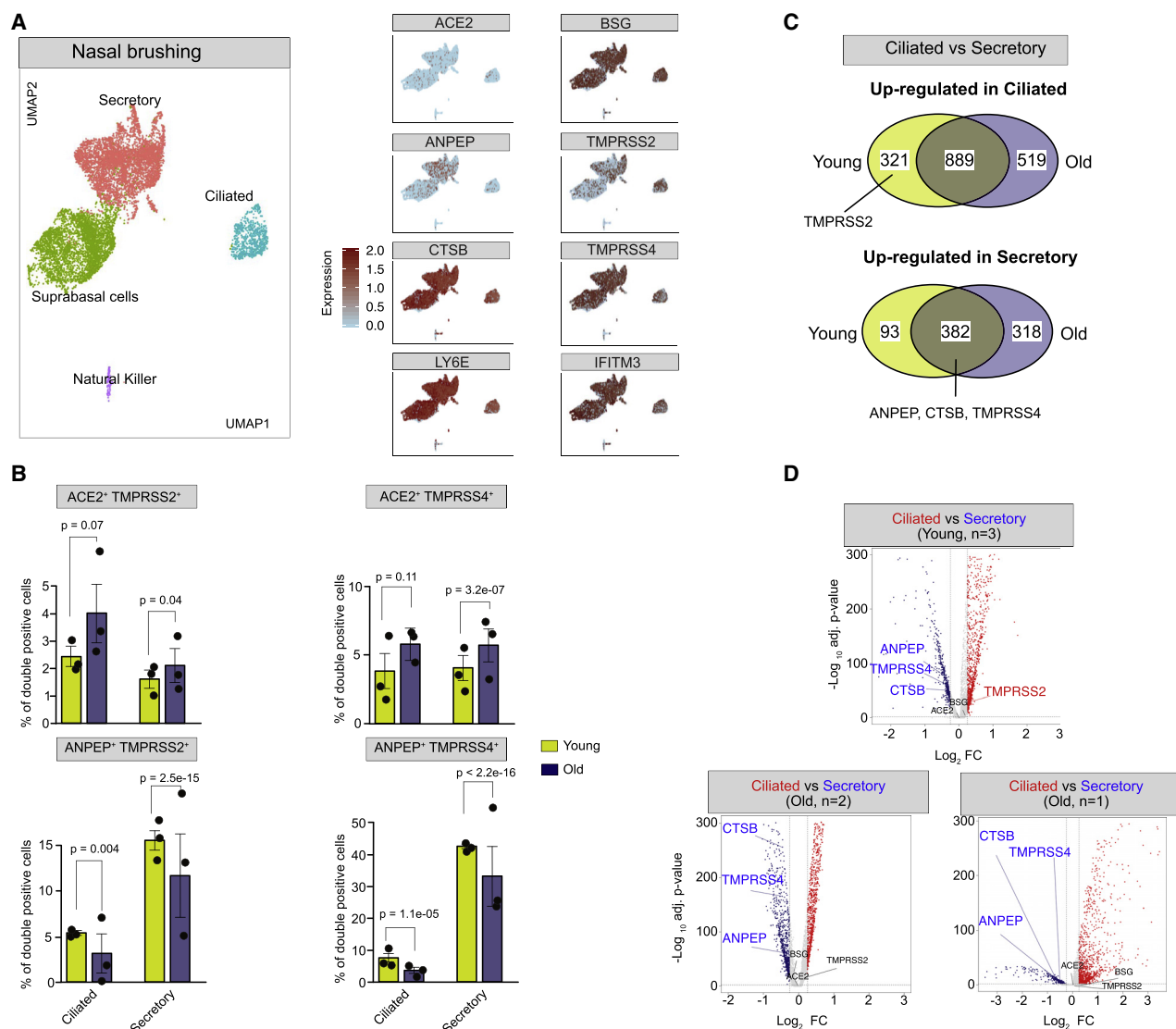
Figure 5. SCARF Expression in Nasal Brushing Samples
