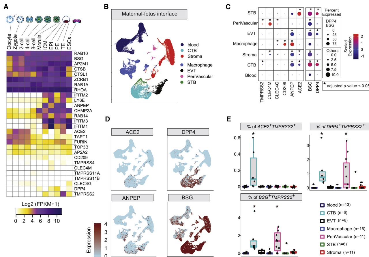
Figure 2. SCARF Expression in Preimplantation Embryo and at the MFI
