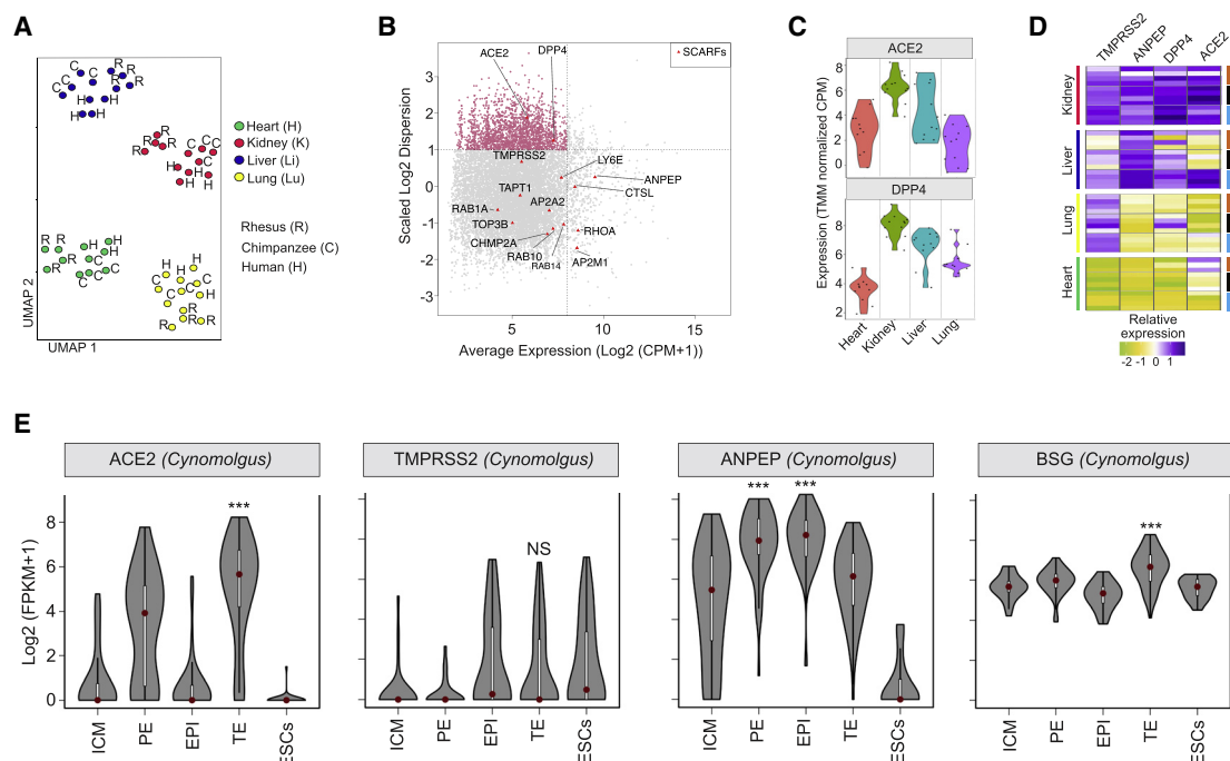
Figure 6. Cross-species Analysis of SCARF Expression
