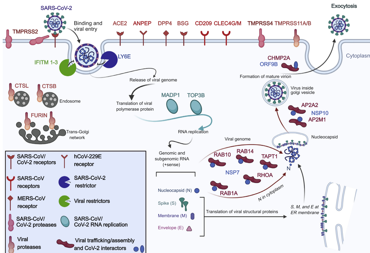
Figure 1. SARS-CoV-2 and SCARFs
