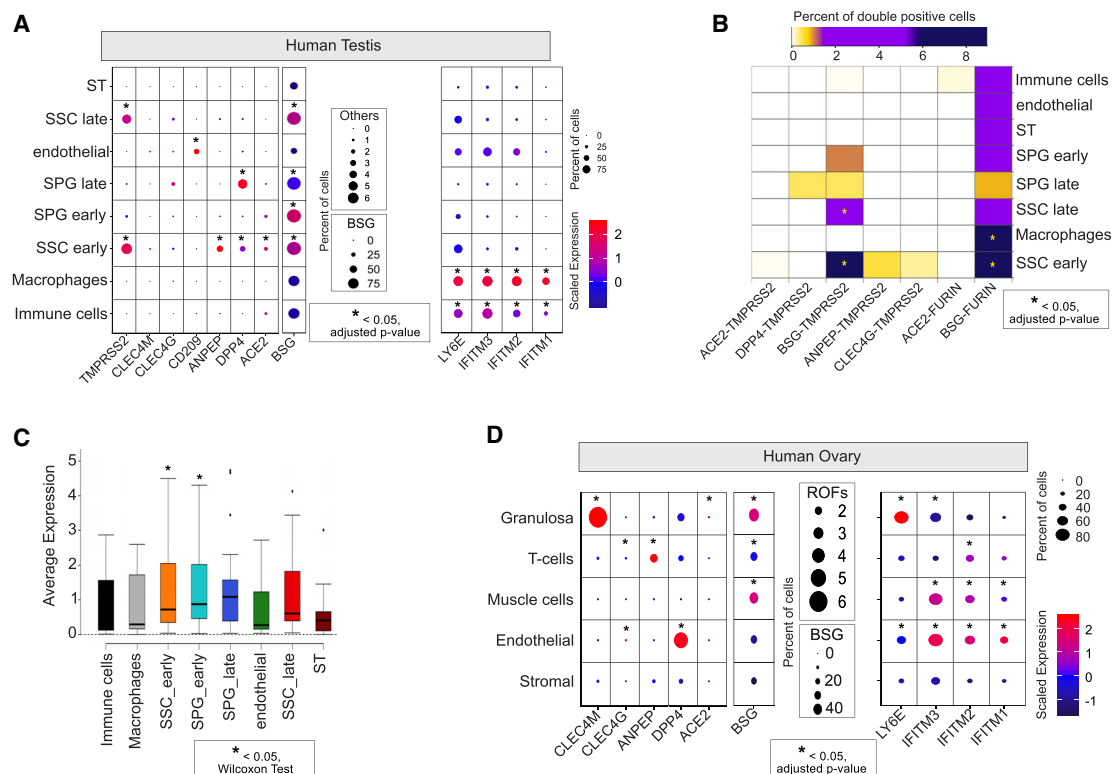
Figure 3. SCARF Expression in Reproductive Organs
