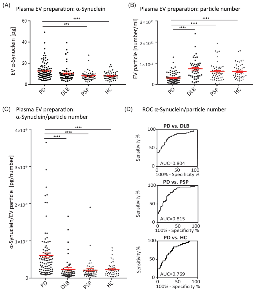
FIG. 2. Characterization of plasma EV α-synuclein in the Tübingen cohort. (A) EV α-synuclein content was determined by electrochemiluminescence analysis and normalized to 1 mL of plasma preparation volume. PD, Parkinson's disease; DLB, dementia with Lewy bodies; PSP, progressive supranuclear palsy; HC, healthy control. Red: mean ± SEM. *** P < 0.0003 , **** P < 0.0001 . (B) EV particle concentration was quantified by NTA from the plasma EV preparation and normalized to 1 mL of plasma preparation volume. PD, Parkinson's disease; DLB, dementia with Lewy bodies; PSP, progressive supranuclear palsy; HC, healthy control. Red: mean ± SEM. **** P = 0.0001 . (C) Ratio of EV α-synuclein to the number of EV particles in the preparation (EV α-synuclein concentration). PD, Parkinson's disease; DLB, dementia with Lewy bodies; PSP, progressive supranuclear palsy; HC, healthy control. Red: mean ± SEM. **** P = 0.0001 . (D) Receiver operating curve (ROC) of the EV α-synuclein concentration to distinguish PD from DLB (upper), from PSP (middle), and from HC (lower). AUC, area under the curve. [Color figure can be viewed at wileyonlinelibrary.com ]
