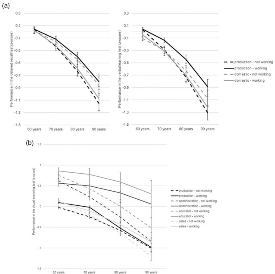
Figure 2. Predicted score in the visual scanning task by working status and occupation in interaction with ageing, as predicted by the mixed models using age as the time variable and with random effects for education and the propensity score.
