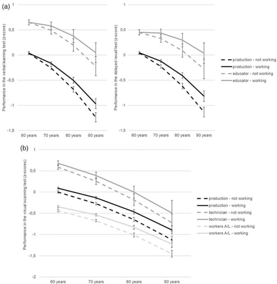
Figure 1. Predicted score in the cognitive tests by working status and occupation, as predicted by the mixed models using year as time and with random effects for education and the propensity score. Note: A/L: agriculture or livestock.
