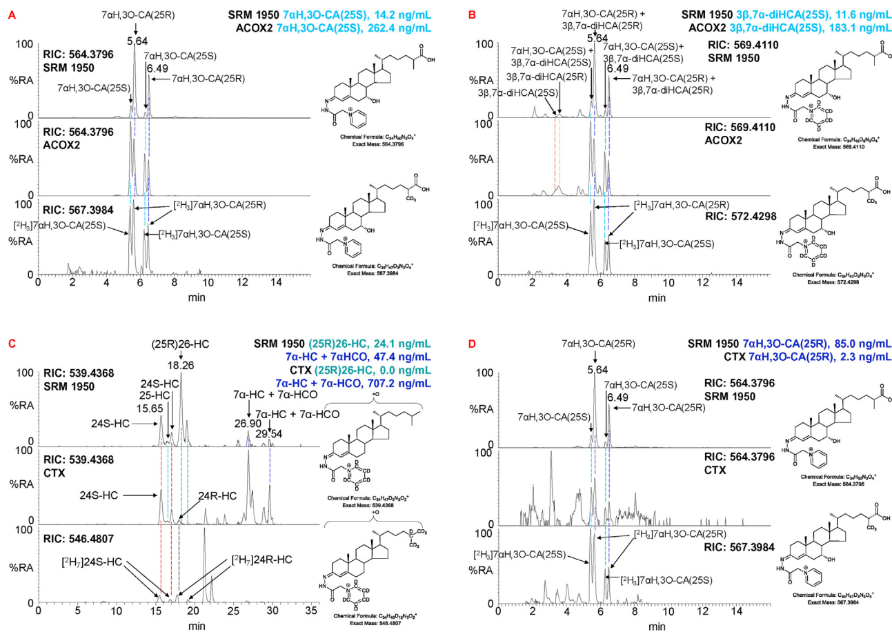
Fig. 5. LC-MS separation of GP-derivatised cholesteric acids, monohydroxycholesterols and monohydroxycholestenones in plasma samples representative of the inborn errors of cholesterol metabolism ACOX2 deficiency and CTX. (A) RIC ( 564.3796 \pm 5 ppm) for [M]^+ ions corresponding to 7\alpha H,30\text{-CA}(25R/S) in NIST SRM 1950 plasma (upper panel), from a patient suffering from ACOX2 deficiency (central panel), and the RIC ( 567.3984 \pm 5 ppm) corresponding to the [M]^+ ion of [^2H_3]7\alpha H,30\text{-CA}(25R/S) (lower panel). (B) RIC ( 569.4110 \pm 5 ppm) for [M]^+ ions corresponding to 3\beta,7\alpha\text{-diHCA}(25R/S) + 7\alpha H,30\text{-CA}(25R/S) in NIST SRM 1950 plasma (upper panel), from a patient suffering from ACOX2 deficiency (central panel), and the RIC ( 572.4298 \pm 5 ppm) corresponding to the [M]^+ ion of [^2H_3]7\alpha H,30\text{-CA}(25R/S) (lower panel). Samples in (A) have been treated with [^2H_0]GP and those in (B) with [^2H_5]GP . (C) RIC ( 539.4368 \pm 5 ppm) for [M]^+ ions corresponding to monohydroxycholesterols and monohydroxycholestenones in NIST SRM 1950 plasma (upper panel), from a sample from a patient suffering from CTX (central panel), and the RIC ( 546.4807 \pm 5 ppm) corresponding to the [M]^+ ion of [^2H_7]24R\text{-S-HC} (lower panel). (D) RIC ( 564.3796 \pm 5 ppm) for [M]^+ ions corresponding to 7\alpha H,30\text{-CA}(25R/S) in NIST SRM 1950 plasma (upper panel), from a sample from a patient suffering from CTX (central panel), and the RIC ( 567.3984 \pm 5 ppm) corresponding to the [M]^+ ion of [^2H_3]7\alpha H,30\text{-CA}(25R/S) (lower panel). Coloured dashed lines indicate the coincidence of oxysterols between chromatograms.
