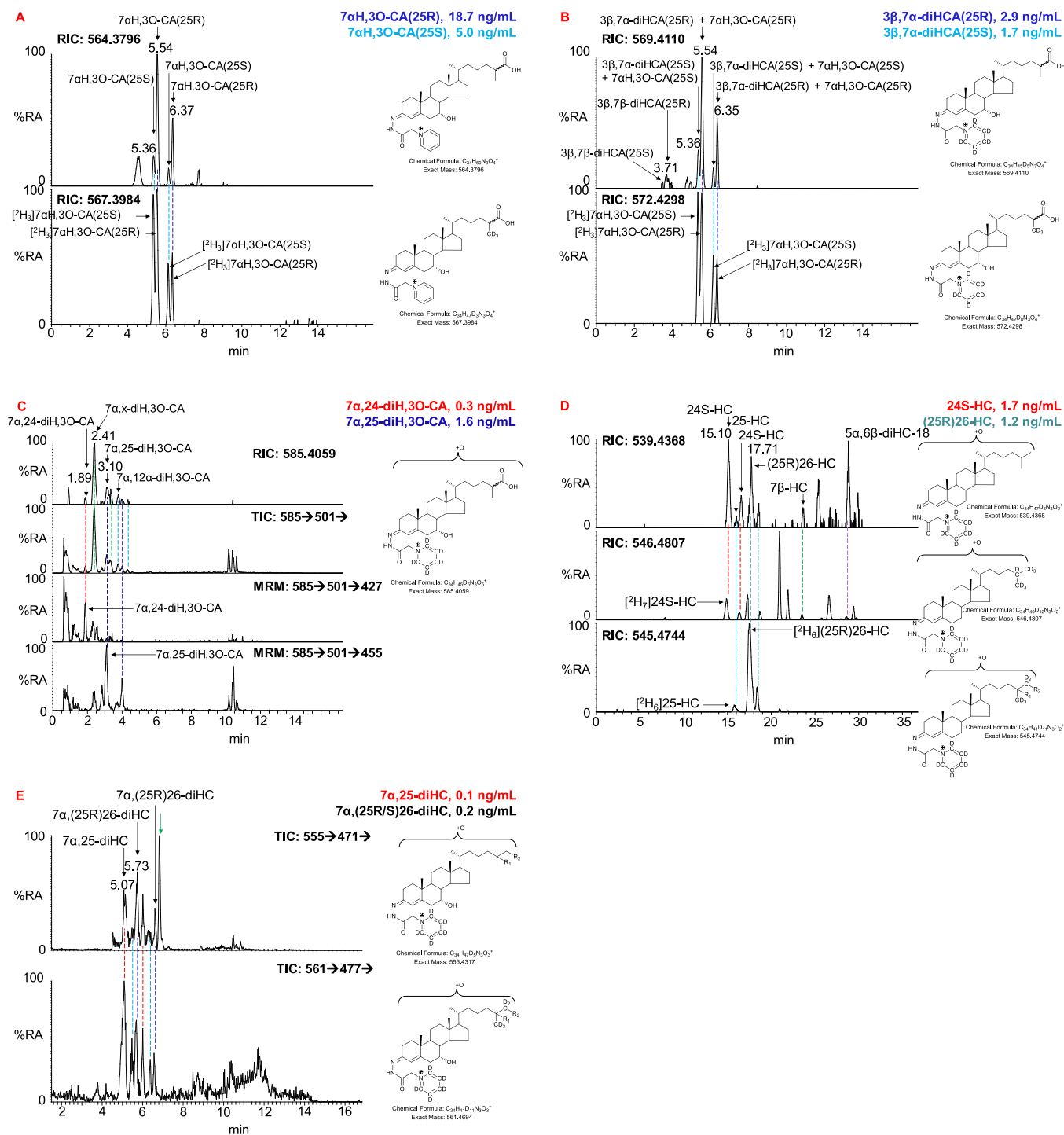
Fig. 4. LC-MS separation of GP-derivatised cholestenic acids, and mono- and dihydroxycholesterols in CSF. (A) RIC for the [M]^+ ions of (upper panel) 7αH,3O-CA(25R/S) ( 564.3796 \pm 5 ppm) found in CSF, and (lower panel) [^2H_3]7\alpha H,3O-CA(25R/S) ( 567.3984 \pm 5 ppm). (B) RIC for the [M]^+ ions of (upper panel) 7αH,3O-CA(25R/S) + 3β,7α-diHCA(25R/S) ( 569.4110 \pm 5 ppm) found in CSF, and (lower panel) [^2H_3]7\alpha H,3O-CA(25R/S) ( 572.4298 \pm 5 ppm). In (A) the derivatisation agent was [^2H_0]GP and in (B) [^2H_5]GP . (C) RIC for the [M]^+ ions of diH,3O-CA isomers ( 585.4059 \pm 5 ppm) found in CSF (upper panel), note the triHCA equivalents are absent. TIC for the MS^3 fragmentation ( 585.4 \rightarrow 501.3 \rightarrow ) for diH,3O-CA isomers (2nd panel). MRM ( 585.4 \rightarrow 501.3 \rightarrow 427.3 ) targeting 7α,24-diH,3O-CA (3rd panel), and MRM ( 585.4 \rightarrow 501.3 \rightarrow 455.3 ) targeting 7α,25-diH,3O-CA (bottom panel). See Supplemental Figures S4P & S4Q for relevant fragmentation schemes. Chromatograms in (A–C) are for non-hydrolysed CSF. (D) RIC of the [M]^+ ions of monohydroxycholesterols ( 539.4368 \pm 3 ppm) found in CSF (upper panel). RIC ( 546.4807 \pm 3 ppm) for [^2H_7]24R/S-HC , [^2H_7]7\beta-HC , [^2H_7]7\alpha-HC and dehydrated [^2H_7]5\alpha,6\beta-diHC (central panel). RIC ( 545.4744 \pm 3 ppm) for [^2H_6]25-HC and [^2H_6](25R)26-HC (lower panel). (E) TIC for the MS^3 fragmentations ( 555.4 \rightarrow 471.4 \rightarrow ) of 7α,25-diHC and 7α,(25R/S)26-diHC found in CSF (upper panel) and for the fragmentations ( 561.5 \rightarrow 477.4 \rightarrow ) of [^2H_6]7\alpha,25-diHC and [^2H_6]7\alpha,(25R/S)26-diHC . Chromatograms (D & E) are for hydrolysed CSF. Coloured dashed lines indicate the coincidence of peaks of the same oxysterol. All chromatograms were recorded over a 17 min gradient.
