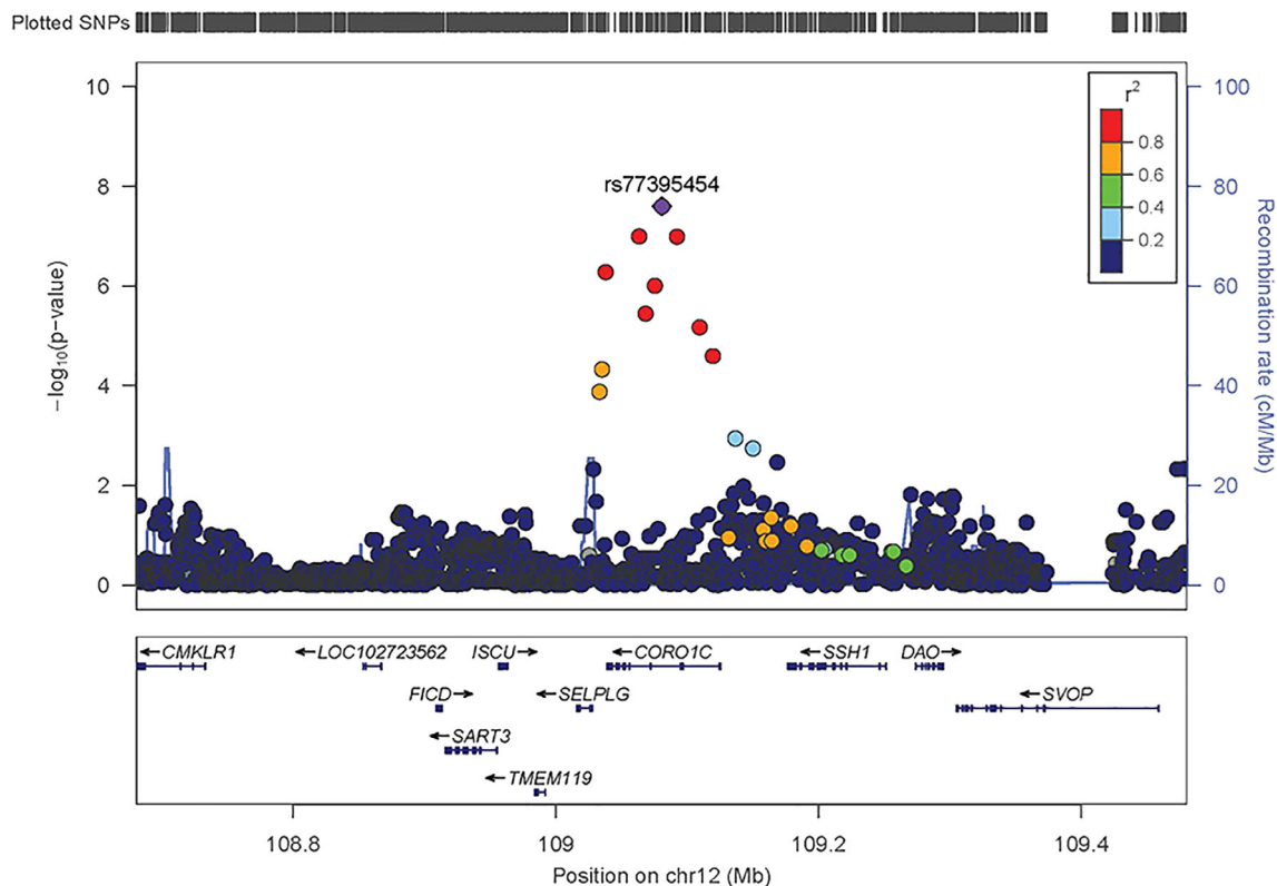
FIGURE 2: Regional association plot of the chromosome 12 region for the penetrance model. Y-axis is the -\log(p \text{ value}) for associations. X-axis denotes physical positions on the chromosome (Mb). The color scale shows the extent of linkage disequilibrium (LD; as measured by r^2 ) between each variant and the top variant (indicated by the purple diamond) with larger r^2 indicating greater LD. Peaks indicate the recombination hot spots. SNP = single nucleotide polymorphism.
