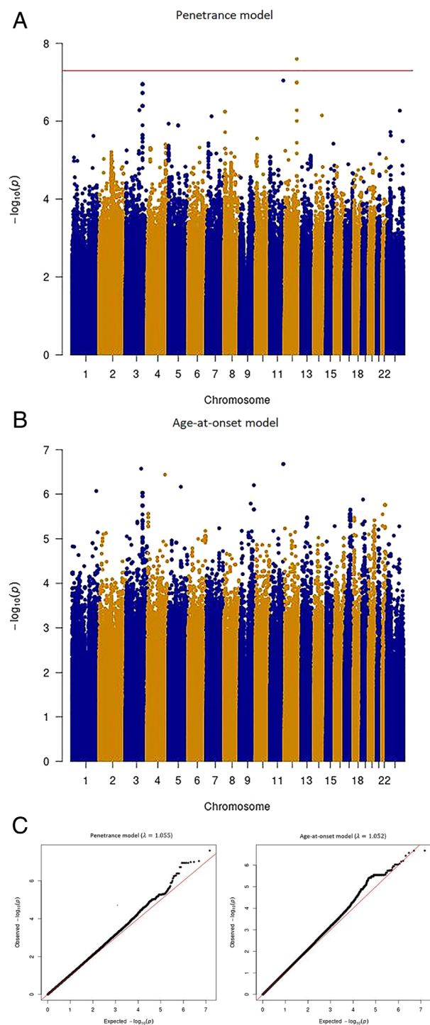
FIGURE 1: Manhattan and Q-Q plots of single variant analysis of penetrance and age-at-onset models. Y-axis is the -\log(p) value for associations. X-axis is physical position of the variants across the genome. The horizontal line indicates genome-wide significance. (A) Penetrance model; (B) age-at-onset model; and (C) Q-Q plots of penetrance model (left) and age-at-onset model (right).
