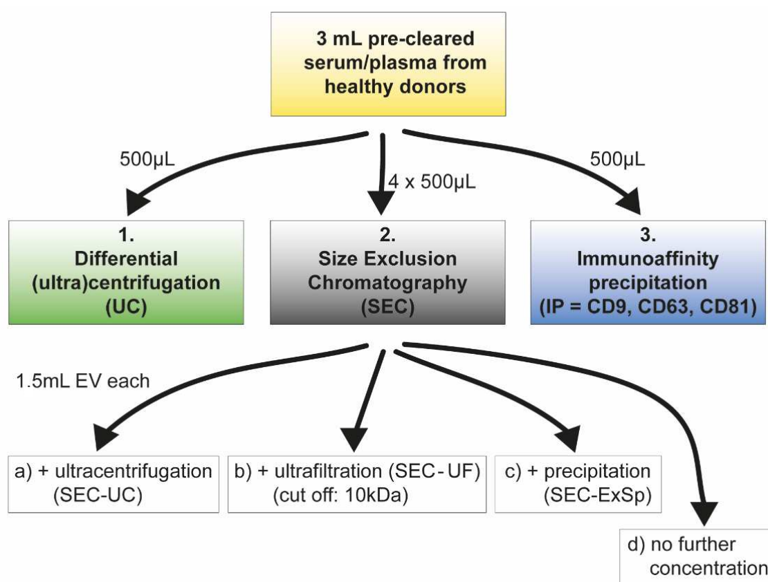
Figure 1. Schematic summary of EV isolation workflow. A total of 3 mL serum or plasma was precleared and split into 500 µL aliquots for subsequent EV isolation with (1) differential (ultra)centrifugation (UC), (2) size exclusion chromatography (SEC), or (3) immunoaffinity precipitation (IP). SEC was performed four times with 500 µL plasma/serum each. Collected fractions (8–10) were first pooled ( 4 \times 1.5 \text{ mL} = 6 \text{ mL} ), and 1.5 mL aliquots EV suspension was used for each following concentration step.
