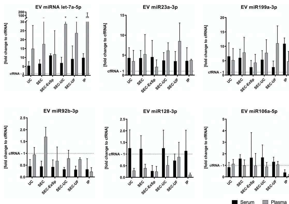
Figure 6. miRNA expression levels in EVs according to the different separation and concentration methods. Depicted is the fold-change of each miRNA compared to the total RNA from cell-free serum/plasma of three healthy volunteers. No significant differences between the EV separation methods were observed, but there was a high and significant variability between individuals for 4 out of 6 miRNAs (let-7a-5p: p = 0.002 , miR-92b-3p: p = 0.01 , miR-199a-3p: p = 0.01 , and miR-128-3p: p = 0.001 ; two-way ANOVA). Note that let-7a-5p, miR-23a-3p, and miR-199a-3p consistently showed higher levels in EVs compared to the corresponding cell-free samples, as opposed to miR-92b-3p and miR-128-3p.
