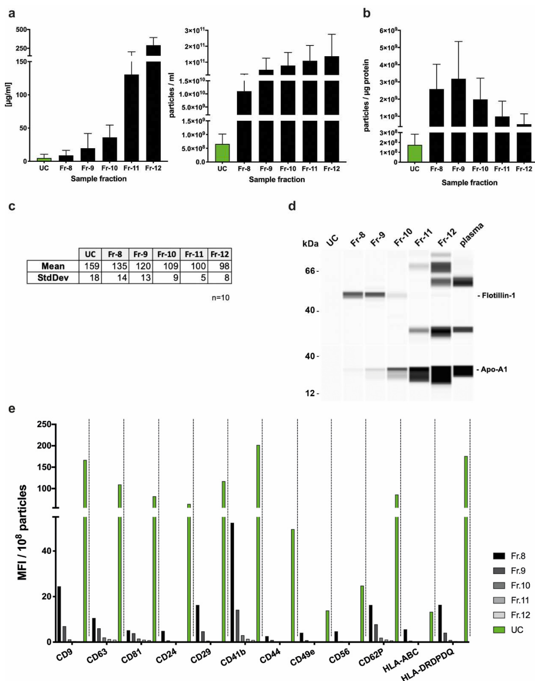
Figure 2. EV yield and characteristics of plasma-derived EV isolated by UC or SEC. (a) Yield of EVs from UC-EVs and SEC-EV fractions 8–12 was determined by overall protein concentration (micro-BCA assay) and particle concentration (determined by NTA). (b) Calculation of the particle number per \mu\text{g} protein, which shows SEC fractions 8–10 to be the EV-containing fractions. (c) Nanoparticle tracking analysis (NTA) of isolated EVs demonstrated that EV size was within the expected range of 100–160 nm. (d) Immunodetection of the EV marker flotillin-1 (and TSG101, Figure S1a) and Apo-A1 as indicator for lipoprotein co-isolation. (e) Surface protein analysis with the MACSPlex assay. Depicted is one representative experiment of 10. The signals are normalized to particle numbers. (MFI—mean fluorescent intensity, SEC—size exclusion chromatography, UC—ultracentrifugation).
