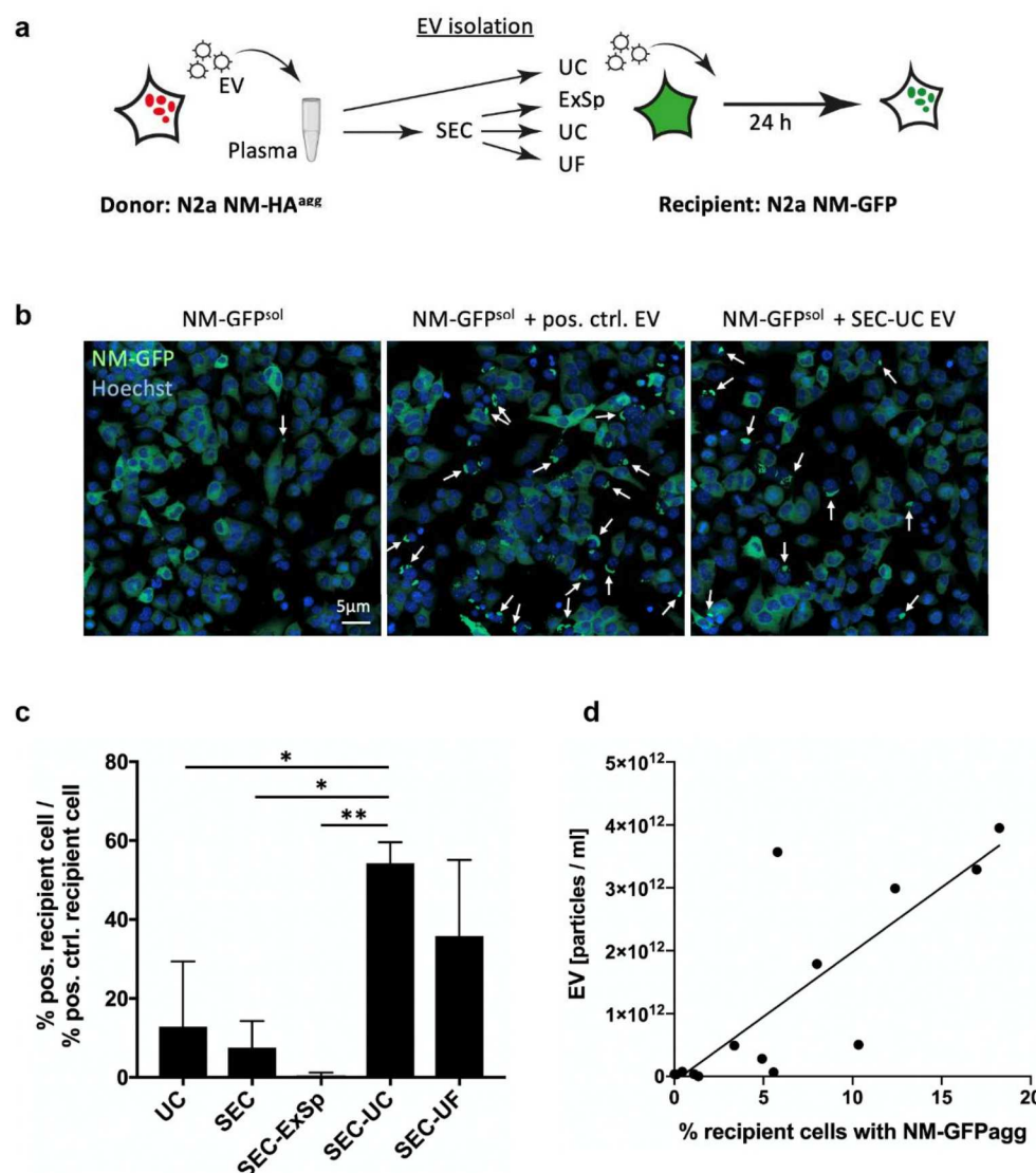
Figure 7. Analysis of isolation-method-dependent differences in EV function (a) Experimental design. EVs containing small NM aggregates from a donor neuroblastoma cell line producing NM-HA aggregates (N2a NM-HA agg ) were collected and spiked into human plasma. EVs isolated by different methods adjusted to similar volumes were subsequently added to recipient reporter cell line expressing soluble NM-GFP (N2a NM-GFP sol ). Uptake of EVs from donor cells results in induction of NM-GFP aggregation (NM-GFP agg ), assessed by automated confocal microscopy. (b) Example Z stack images of recipient reporter cell line before (left) and after exposure to donor EVs (middle) or spiked EV isolated by SEC-UV (right). Nuclei were stained with Hoechst. White arrows indicate NM-GFP aggregate formation. (c) Reporter NM-GFP agg induced by exposure of recipient N2a NM-GFP sol cells to spiked EVs. Shown are the percentages of recipient cells with induced NM-GFP agg 24 h post exposure to EVs. Aggregate induction by spiked plasma EV samples relative to induction by non-spiked UC-EVs from donor cells is shown. SEC + UC EVs isolation resulted in highest percentage of cells with NM-GFP agg (* p < 0.05 , ** p < 0.01 , two-way ANOVA; n = 3 independent experiments). (d) Spearman correlation of NM-GFP aggregate formation and concentration of all EVs irrespective of the isolation method. A high correlation between parameters was found (Spearman r = 0.85 (95% CI: 0.561–0.952), p = 0.0003 ).
