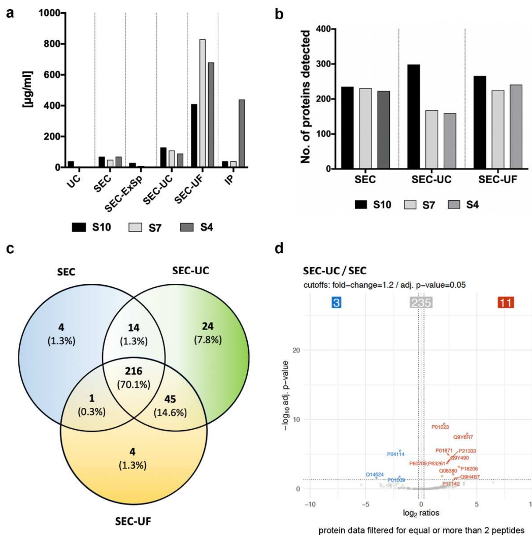
Figure 5. Variable protein detection depending on the EV isolation method ( a,b ) Differences in protein concentration and protein detection of EVs separated by different methods from human serum of three healthy volunteers (S10, S7, and S4). The highest protein concentration was obtained with SEC-UF (two-way ANOVA: p = 0.0002 , reference: UC). ( c ) Representative Venn diagram (from volunteer S10) of proteins detected with SEC alone or when followed by concentration with UC and UF. Note the high number of shared proteins ( n = 216 , 70.6%) and that 24.7% of the proteins were detectable only after concentrating the EV sample with either UC or UF. ( d ) Significant, differentially identified proteins with SEC and SEC-UC. When applying filters of q < 0.05 and a fold-change of at least 1.2 (shown with dotted lines), only 14/256 proteins were differentially identified. Out of these, only 9 proteins showed an up- or down-regulation in at least 2/3 samples (see Table 1A). In total, 14 proteins were detected at different levels in SEC and SEC-UC, out of which n = 11 differed significantly in at least 2/3 donors ( n = 6 increased and n = 3 decreased in SEC-UC compared to SEC). The six significantly increased proteins in SEC-UC vs. SEC were mainly Ig-related or structural proteins. In SEC-UF, three apolipoproteins were significantly reduced compared to SEC alone in at least 2/3 donors (Table 1).
