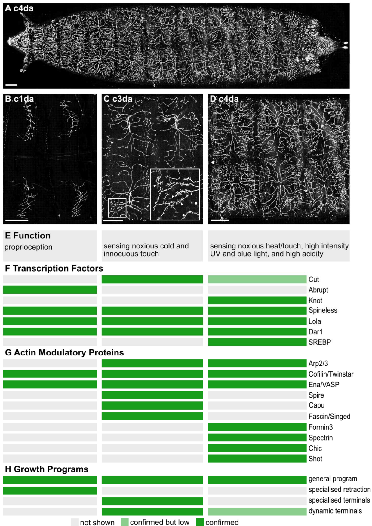
Figure 1. Structure and function of da neurons. (A–D) Living wandering third instar larvae were immobilized in between a
