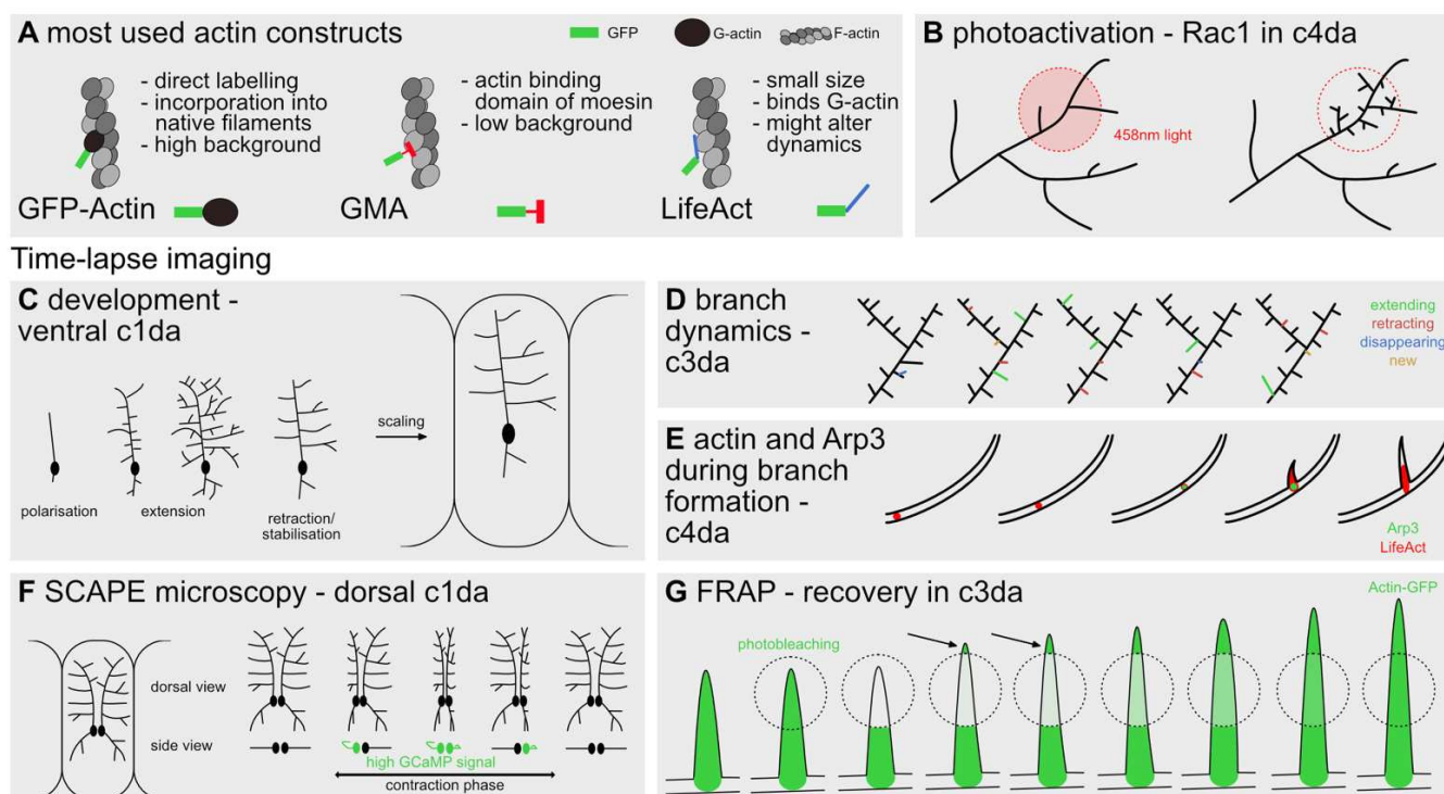
Figure 2. Tools for in vivo imaging and manipulation. (A) The three most commonly used constructs for visualizing actin in vivo. Schemes show how GFP-actin, GMA and LifeAct are incorporated into an actin filament. (B) Example of how a photoactivatable construct can help understanding the functional role of a specific molecule or cascade in dendrites. PA Rac1 activation in c4da neurons with blue light (458 nm) leads to the formation of small dendritic branchlets [27]. (C–G) Examples of how time-lapse imaging was used to understand different stages of dendrite branch formation. (C) Long-term imaging of the c1da neurons throughout embryonic and larval development, elucidating the sequence of differentiation stages [12,15]. (D) High-resolution imaging in the terminal branches of c3da neurons to analyze their constant dynamics. Analysis of branches newly forming, extending, retracting, and disappearing can be monitored within a range of 30 min [13]. (E) Dynamics of actin patches (LifeAct, here shown in red) along dendritic branches of c4da neurons, accumulating before new branch formation and extending into the newly formed branchlet [26]. Labeled Arp3 (shown as a green dot) accumulates transiently at the site before a new branch is formed and disappears shortly after branch formation [27]. (F) High-speed imaging of c1da neurons with SCAPE microscopy allows monitoring the deformation and the intracellular calcium activity of the dendrites in freely moving larva [36]. (G) Bleaching and subsequent recovery of the GFP-actin signal at the tip of a growing dendritic branchlet of a c3da neuron. The most commonly used bulk kinetics approach method to study actin structure was performed in vivo to define the orientation of actin filaments in the extending branchlet [13].
