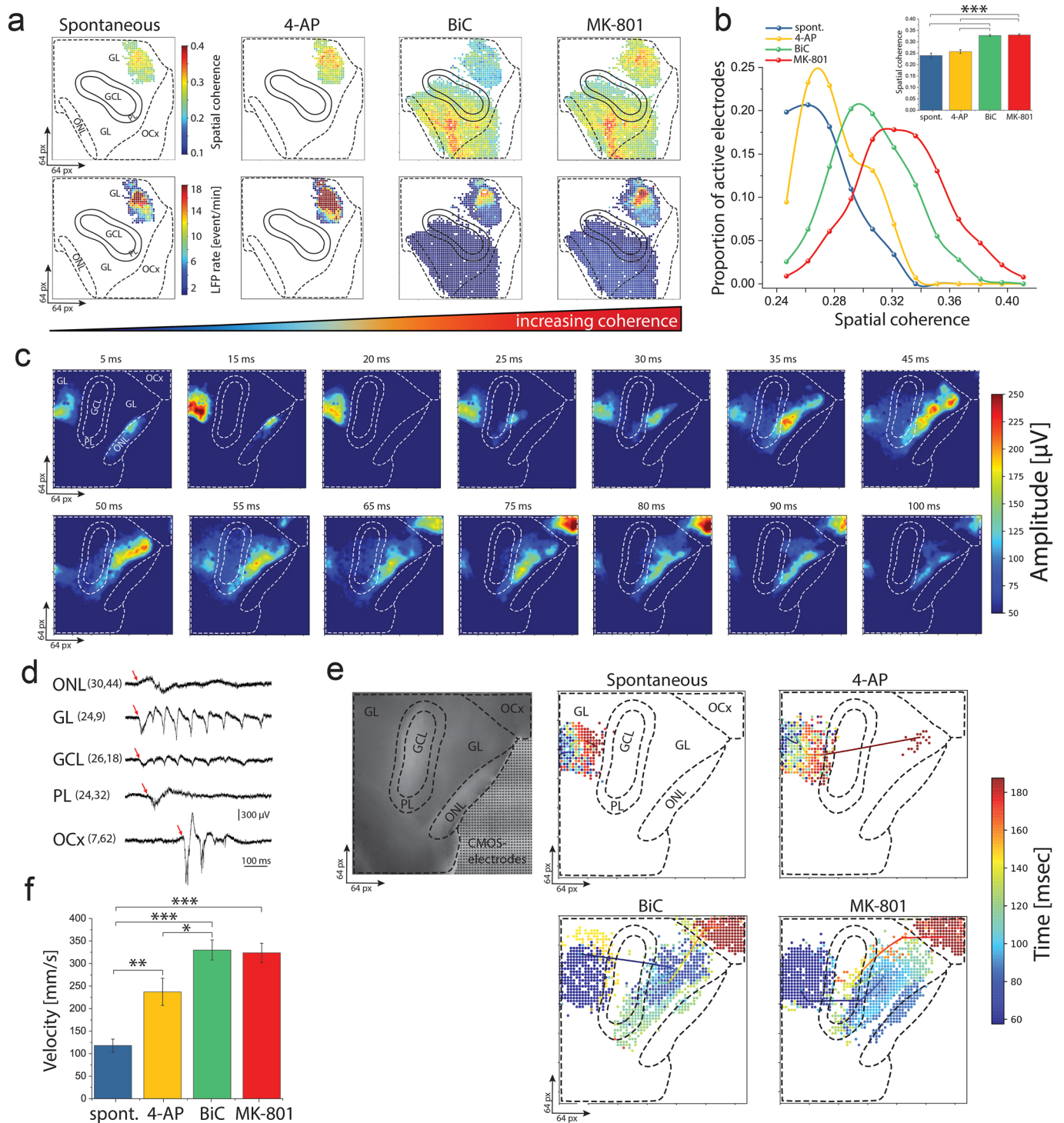
Fig. 4. Topographical analysis of spatiotemporal dynamics of coding information. a) Spatial coherence maps displaying correlated pairs of recorded sites in the OB circuit. Maps on top showing the coherence, and at the bottom are the maps of firing information encoded in field potentials. Spatial coherence increasing sequentially by pharmacological treatment of 4-AP, BiC, and MK-801, respectively, yielding more active electrodes encoding higher information of the firing rate of that spectral frequency component (i.e., in the GL). b) Spatial coherence quantification showing a significantly shifted distribution towards higher coherence values under drug-treatment compared with spontaneous activity and summarized in (b, inset) (** p < 0.001 , ANOVA, n = 24 slices from 8 mice). c) Profile of propagation sequence of representative LFP event showing a defined initiation (ONL and GL) and dynamic propagation of the LFP firing patterns in the OB interconnected circuitry (sending output at the OCx). d) Temporal event traces corresponding to active recording sites in different OB layers. The red arrows point to the initiation time and shift to the right to indicate the propagation sequence (i.e., initiated in ONL-GL and terminates at OCx). e) Averaged CATs superimposed to the propagating active electrodes and the morphological structure of the OB layers. Time color-coded scale (right) indicates the CATs propagation profile and the firing electrodes of a single LFP event. f) Velocity of conduction of propagating LFP events is significantly increased when recording performed with 4-AP, BiC, and MK-801 compared to spontaneous (* p < 0.05 , ** p < 0.01 , *** p < 0.001 ANOVA, n = 24 slices from 8 mice). (For interpretation of the references to color in this figure legend, the reader is referred to the Web version of this article.)
