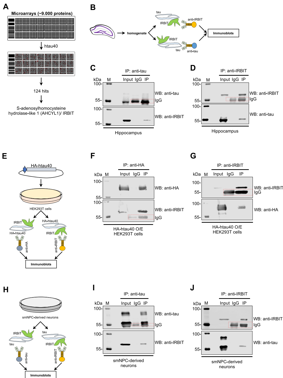
Figure 1. AHCYL1/IRBIT binds tau. A , schematic representation of the human protein–protein microarray approach. Using 5 and 50 ng/μl of recombinant full-length human tau, we identified 124 tau-interacting polypeptides, including AHCYL1/IRBIT. B , scheme and ( C and D ) WBs of immunoprecipitated proteins from mouse adult hippocampi. Immunoblots were developed using anti-tau and anti-IRBIT antibodies. E , scheme and ( F and G ) WBs of immunoprecipitated proteins from HEK293T cells transiently transfected with a plasmid encoding HA-tagged htau40. After 48 to 72 h, cells were harvested, crosslinked, and lysed. Co-IPs were performed using an antibody against ( F ) HA and ( G ) IRBIT. H , scheme of IP strategy and ( I and J ) WBs of immunoprecipitated proteins from smNPC-derived neuronal cultures. Co-IPs were performed using antibodies against ( I ) tau and ( J ) IRBIT. Immunoblots were developed using the antibodies indicated on the right. Red dotted rectangles indicate bands because of IgG. M is protein molecular marker. AHCYL1/IRBIT, SAH hydrolase–like protein 1/IP3R-binding protein; co-IP, coimmunoprecipitation; HA, hemagglutinin; HEK293T, human embryonic kidney 293T cell line; IgG, immunoglobulin G; smNPC, small-molecule neural progenitor cell; WB, Western blot.
