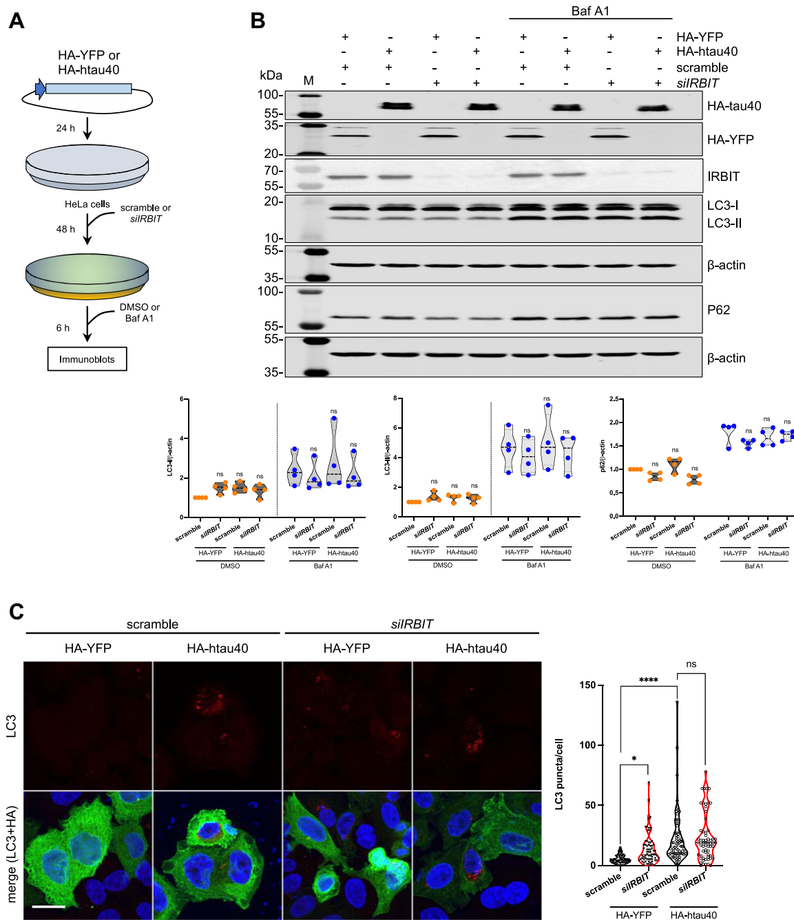
Figure 5. Tau overexpression may influence autophagy in HeLa cells. A, schematic representation of the experimental setup. HeLa cells were transfected with HA-YFP or HA-htau40, followed by retransfection with scramble or siIRBIT . After 48 h, cells were incubated with DMSO or 100 nM bafilomycin A1 for 6 h. B, representative immunoblot for autophagy-related proteins LC3-I, LC3-II, and p62 in transfected HeLa cells. M is protein molecular marker. Quantification of LC3-I, LC3-II, and p62 protein levels normalized to β-actin. Densitometry is on the bottom. C, representative confocal images of HeLa cells overexpressing HA-YFP or HA-htau40 (green) stained for LC3-positive puncta (red). Nuclei (blue) were stained with Hoechst-33342. The scale bar represents 20 μm. The graph shows quantification of LC3-positive puncta per cell. Data in B and C were statistically analyzed via one-way ANOVA followed by Dunnett's multiple comparisons test (**** p < 0.0001 , * p < 0.05 , ns). DMSO, dimethyl sulfoxide; HA, hemagglutinin; ns, not significant.
