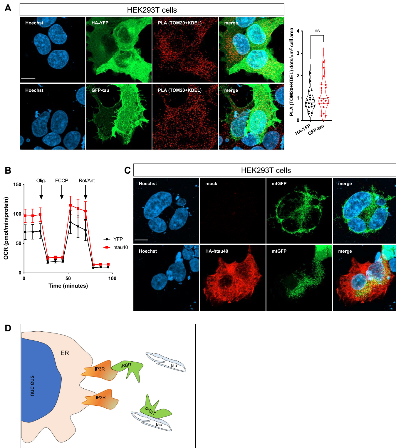
Figure 4. Tau overexpression alters neither mitochondria-ER contact sites nor mitochondrial respiration. A , representative confocal images of HA-YFP and GFP-tau overexpressing HEK293T cells stained with PLA (TOM20 + KDEL). Quantification of PLA dots is shown on the right . Data were obtained from two independent experiments and n = 19 cells/condition (unpaired t test, ns). The scale bar represents 10 \mu\text{m} . B and C , seahorse analysis and representative confocal images of HEK293T overexpressing mitochondrial-targeted GFP and GFP-tau. The scale bar represents 10 \mu\text{m} . D , schematic representation of the interaction between tau, IRBIT, and IP3R. As a result of tau binding, IRBIT dissociates from IP3R at the ER. ER, endoplasmic reticulum; HA, hemagglutinin; HEK293T, human embryonic kidney 293T cell line; IP3R, inositol 1,4,5-trisphosphate receptor; KDEL, Lys-Asp-Glu-Leu; ns, not significant; PLA, proximity ligation assay; TOM20, translocase of outer mitochondrial membrane 20.
