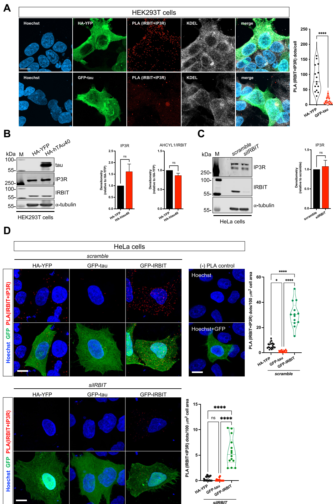
Figure 3. Tau interferes with AHCYL1/IRBIT localization at the IP3R. A, PLA staining in HEK293T cells O/E HA-YFP or GFP-tau using primary antibodies against IRBIT and IP3R. Quantification of PLA dots is shown on the right. Data were obtained from two independent experiments and n = 15 cells/condition (unpaired t test, ****, p < 0.0001 ). The scale bar represents 10 \mu\text{m} . B, representative immunoblots of HEK293T cells overexpressing HA-htau40. M is protein molecular marker. Densitometries for IP3R and AHCYL1/IRBIT expression are on the right ( n of experiments = 4; unpaired t test, ns). C, representative immunoblots of IP3R and AHCYL1/IRBIT in HeLa cells transfected with scramble and siIRBIT . M is protein molecular marker. Densitometry of IP3R expression is on the right ( n of experiments = 4; unpaired t test, ns). D, representative confocal images of HA-YFP, GFP-tau, and GFP-IRBIT overexpressing HeLa cells, which were cotransfected with scramble and siIRBIT . Cells were stained with Hoechst-33342 (nuclei, blue), anti-GFP (green), and PLA (IRBIT + IP3R, red).
