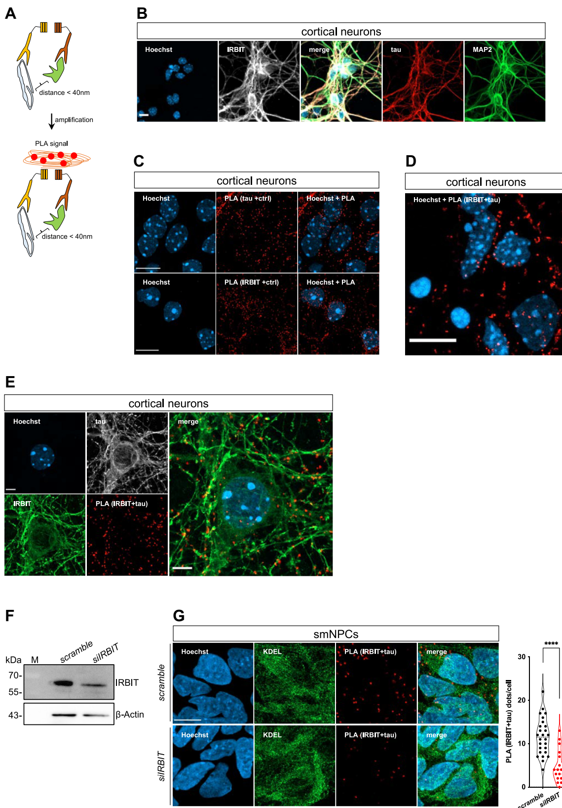
Figure 2. AHCYL1/IRBIT and tau are in close proximity in cultured cells. A , schematic representation of the PLA method. B , confocal images of 7-day-old mouse primary cortical neurons stained with Hoechst-33342 (blue), IRBIT (white), tau (red), and MAP2 (green). The scale bar represents 5 \mu m. C , confocal images of primary cortical neurons stained with Hoechst-33342 (blue) and PLA probe (red). Primary antibodies were against IRBIT and tau, with +ctrl indicating the presence of species-specific secondary antibodies. The scale bar represents 10 \mu m. D , representative PLA (IRBIT + tau) staining in cortical neurons. Hoechst-33342 was used to stain the nucleus. The scale bar represents 10 \mu m. E , confocal images of mouse-derived cortical neurons stained with Hoechst-33342 (blue), tau (white), IRBIT (green), and PLA (IRBIT + tau; red). The scale bar represents 5 \mu m. F , representative immunoblots of smNPCs transfected with scramble and siIRBIT. Antibodies against IRBIT and \beta -actin (as loading control) were used. M is protein molecular marker. G , representative
