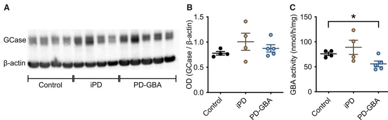
Figure 2 GCCase protein levels and activity in fibroblasts. Measurements were made in fibroblasts from control subjects and idiopathic Parkinson's disease (iPD) and PD-GBA patients. (A) Western blots showing immunoreactivity for human GCCase and \beta -actin (one replicate per cell line). (B) Semi-quantitative analysis of band intensities of the blots shown in A. (C) Measurements of GCCase activity in fibroblasts from the control ( n = 4 ), idiopathic Parkinson's disease ( n = 4 ) and PD-GBA ( n = 5 ) groups (three replicates per cell line). Data are shown as individual values and mean \pm SEM. Unpaired t-test was performed to compare data in control subjects versus values in the idiopathic Parkinson's disease or PD-GBA groups. Control versus PD-GBA: P = 0.0258 ; F(4,3) = 3.734 . * P < 0.05 .
