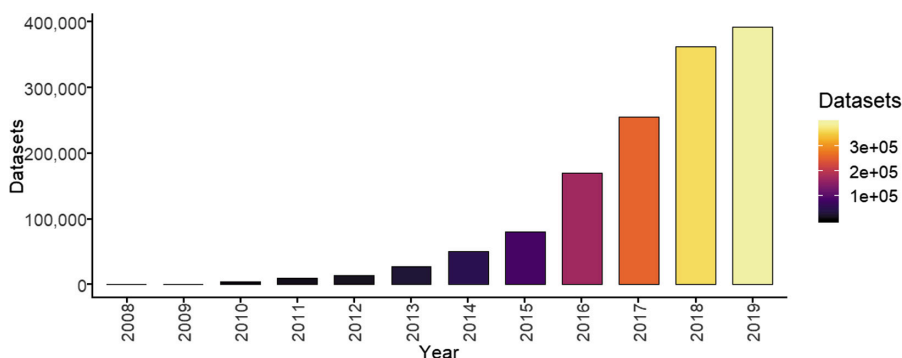
Fig. 1. Number of high throughput sequencing (HTS) data sets uploaded to NCBI per year. The 2019 data is still incomplete, since most studies are only uploaded to NCBI once they are published.
