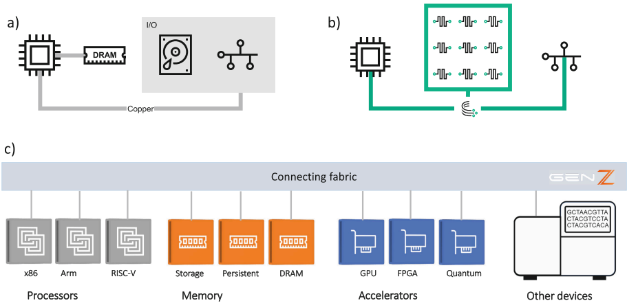
Fig. 2. (a) The traditional von Neumann architecture defines the processor as the central component. (b) MDC puts persistent memory at the center of the system. Components are linked through an optical fabric. (c) The connecting fabric, e.g., Gen-Z, puts different components from the processor-, memory- and accelerator class in a single shared address space. Other specialized devices like sequencers for data generation could also be integrated.
