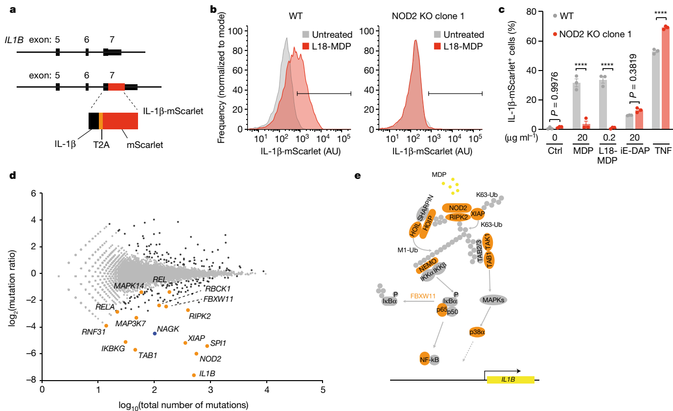
Fig. 1 | A haploid genetic screen reveals regulators of NOD2. a , CRISPR engineering of the IL1B locus, resulting in an endogenous in-frame fusion of IL-1β and mScarlet separated by a self-cleaving peptide (T2A). b , Flow cytometry analysis of IL-1β-mScarlet induction following L18-MDP stimulation of wild-type (WT) and NOD2-knockout (KO) clonal KBM-7-IL-1β mScarlet cells for 16 h. Data shown for one representative of three independent experiments, indicating gating strategy. AU, arbitrary units. c , Flow cytometry analysis of IL-1β-mScarlet induction in wild-type and NOD2-knockout clonal KBM-7-IL-1β mScarlet cells stimulated as indicated for 16 h. Data are mean \pm s.e.m. of n = 3 independent biological samples. Two-way ANOVA with Šidák's multiple-comparisons test. Ctrl, control. d , Genetic screen showing positive
