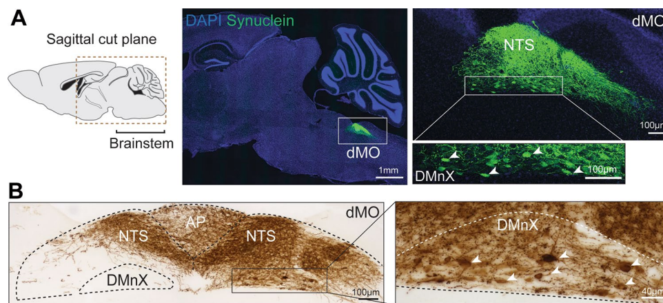
Fig. 1 Targeted overexpression of h \alpha -synuclein in the dorsal medulla oblongata. Images were obtained from mice that received an intravagal injection of h \alpha -synuclein-AAVs and were sacrificed 2 weeks later. A The fluorescent image on the left shows h \alpha -synuclein-containing neurons (green) in the dorsal medulla oblongata (dMO) in a sagittal brain section that was stained with both anti-h \alpha -synuclein and DAPI (blue). The square rectangle delineates an area containing the nucleus of the tractus solitarius (NTS) and the dorsal motor
