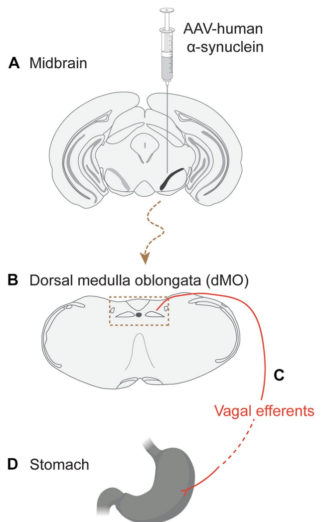
Fig. 3 Schematic representation of long-distance brain-to-stomach \alpha -synuclein spreading. This spreading was initiated by an injection of \alpha -synuclein-AAVs in the rat midbrain ( A ). The exogenous protein first reached the dorsal medulla oblongata (dMO, box delineated by dashed lines) and, in particular, the dorsal motor nucleus of the vagus ( B ). It then traveled through efferent axons of the vagus nerve ( C ) and was finally detected within vagal nerve endings in the gastric wall ( D )
