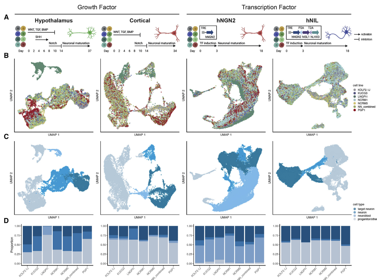
Figure 4. Differentiation potential of candidate cell sub-lines
