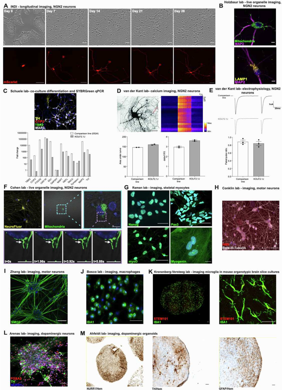
Figure S6. Differentiation and functional evaluation of KOLF2.1J by diverse methods.
