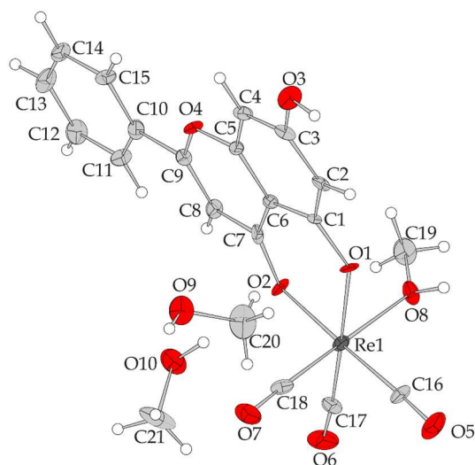
Fig. 3 Structure of [\text{Re}(\text{CO})_3(\text{chrysin})(\text{MeOH})]_2(\text{MeOH}) . Ellipsoids were drawn with 50% probability. Selected bond lengths (Å): \text{Re1—O1}=2.124 (5); \text{Re1—O2}=2.092 (5); \text{Re1—O8}=2.185 (6); \text{Re1—C16}=1.925 (8); \text{Re1—C17}=1.921 (9); \text{Re1—C18}=1.913 (9). Selected angles (°): \text{O1—Re1—O2}=84.2 (2); \text{O1—Re1—O8}=81.4 (2); \text{O2—Re1—O8}=84.4 (2); \text{O2—Re1—C16}=176.5 (3); \text{O1—Re1—C17}=174.0 (3); \text{O8—Re1—C18}=177.3 (3)
