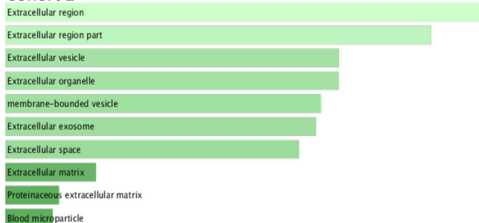
FIGURE 2 (A) All identified proteins in Cohort 1 (lilac) and Cohort 2 (green) enriched for cellular compartment localization led to identification of terms related to extracellular vesicles/exosomes. (B) Overlap of all proteins in Cohort 1 and Cohort 2 with ExoCarta top 100 proteins (yellow).
