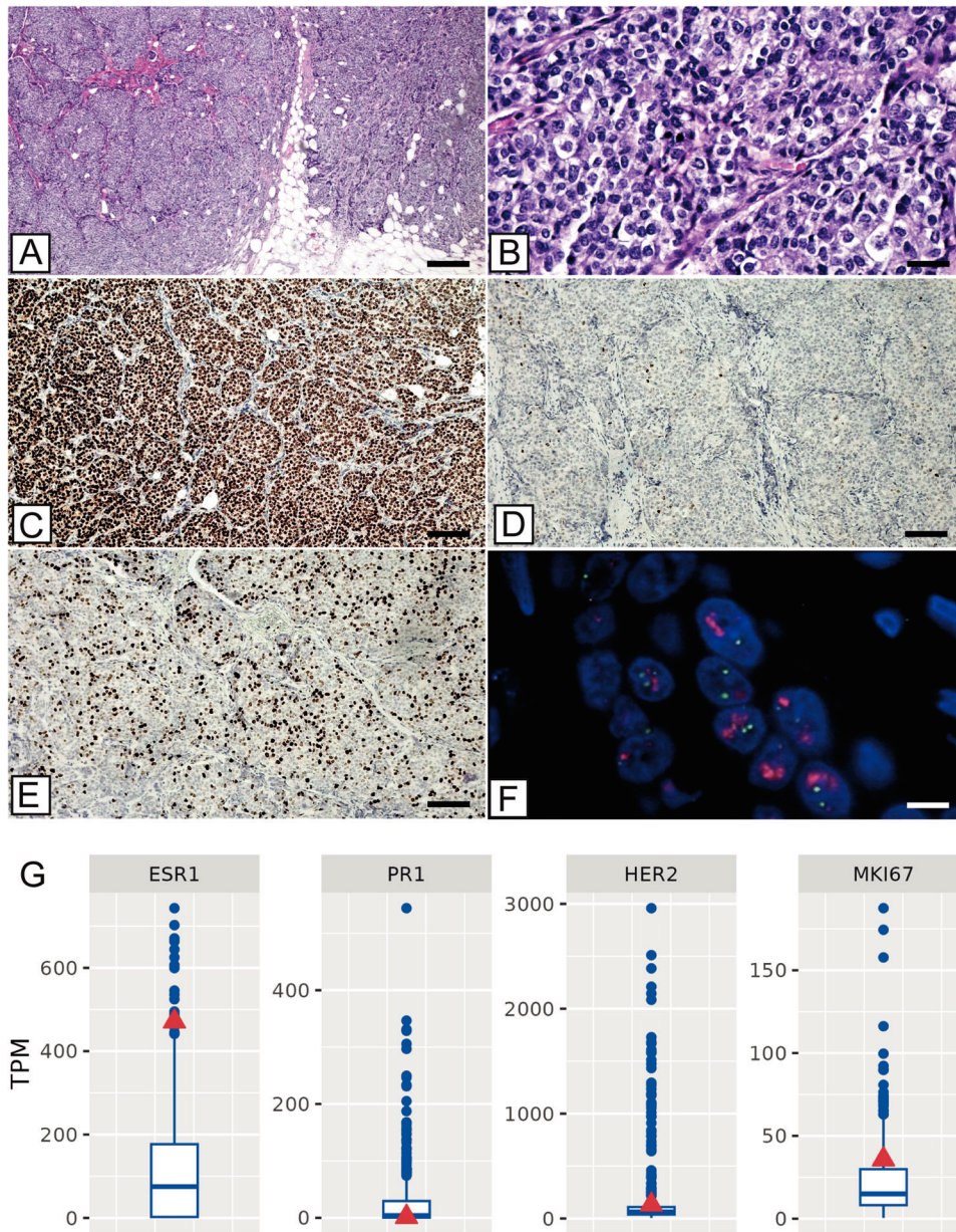
Fig. 1 Histopathological and molecular characterization of the tumor. A Haematoxylin and eosin slide shows a ductal infiltrating breast carcinoma (G3) (scale bar represents 200 \mu\text{m} ). B High magnification of panel A shows high cellular pleomorphism, absence of tubules and numerous mitoses (scale bar represents 20 \mu\text{m} ). C Estrogen receptor expression in more than 95% of breast cancer cells (scale bar represents 200 \mu\text{m} ). D Progesterone receptor expression in about 1% of breast cancer cells (scale bar represents 200 \mu\text{m} ). E Image displays high proliferation index (Ki67 > 35%) (scale bar represents 200 \mu\text{m} ). F In situ hybridization analysis of HER2 status demonstrates the amplification of HER2 gene (ErbB2/CEN17 ratio > 2) (scale bar represents 10 \mu\text{m} ). G Expression mRNA levels (TPM) of estrogen receptor 1 (ESR1), progesterone receptor (PR1), ERBB2 receptor tyrosine kinase 2 (HER2) and proliferation marker KI-67 (MKI67) for the patient (red triangle) and the clinical cohort (blue boxplot).
