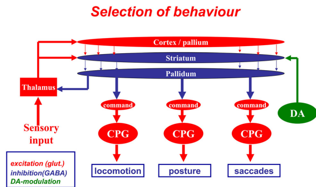
Figure 2: Central pattern generator (CPG) selection. The cortex in mammals and the corresponding structures in lower vertebrates (pallium), alongside the thalamus, provide an excitatory (red) input to striatum. The striatum consists primarily of inhibitory (blue) GABAergic neurons, which in turn inhibit the output nuclei of the basal ganglia (pallidum, and in mammals, the substantia nigra pars reticulata [not shown]), as part of the basal ganglia's direct pathway. The output nuclei again consist of GABAergic neurons, and their high level of baseline activity keeps CPGs elsewhere in the nervous system under tonic inhibition. This is released when the striatum is activated and inhibits the output nuclei, resulting in a disinhibition of the CPGs. Dopamine (DA) affects the responsiveness of striatal neurons. Reproduced with permission from Grillner et al. (2006).
