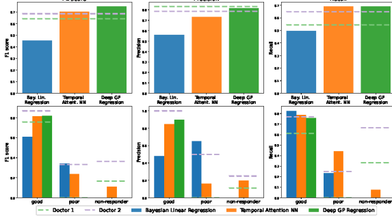
(b) Classification Performance: LMM preprocessed data: n_{visits} = 2
