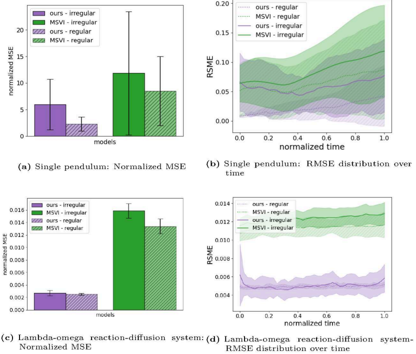
Figure 3.10: Test errors of different models for regular and irregular time grids: (a) Normalized MSE for single pendulum dataset, (b) RMSE over time for single pendulum dataset, (c) Normalized MSE for lambda-omega reaction-diffusion system, (d) RMSE over time for lambda-omega reaction-diffusion system.
