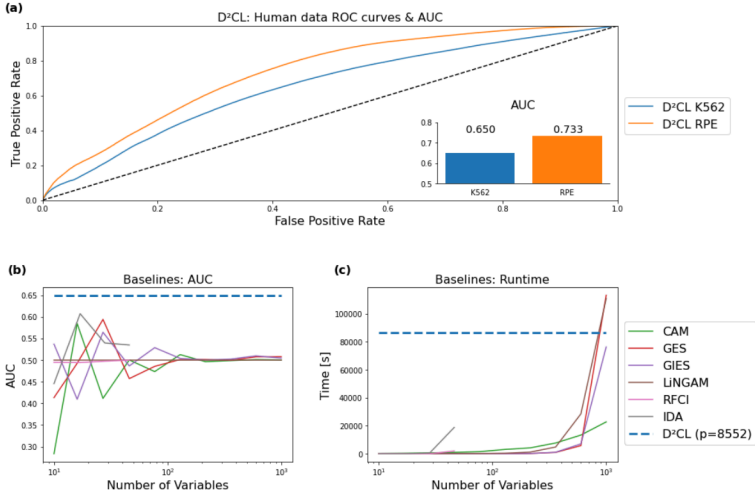
Figure 2.8: Results - high-dimensional human data. Single-cell CRISPR-based experiments (due to [55]) were used to illustrate the use of the proposed approaches in high-dimensional human data. Performance was quantified using causal ROC curves (and the area under the curve, or AUC) computed with respect to a causal ground truth obtained from entirely unseen interventional experiments. (a) Results from D²CL applied to data obtained from retinal pigment epithelial cells (RPE) and a cancer cell line (K562) in problems spanning more than 8000 variables (other methods could not be practically run in this case due to computational burden). (b) Performance of existing causal learning approaches (on K562 data) as a function of problem dimension. The dashed line indicates D²CL performance on the full problem ( p=8552 variables). We see that for the existing methods tested, performance converges to the level of random guessing once more than \sim 100 variables are considered. (c) Computational runtime as a function of problem dimension. (Runtime of D²CL on the full problem with p=8552 including full training and inference is shown as a dashed line; shown only for completeness).
