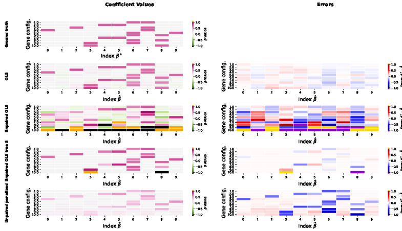
Figure 4.8: RPE gene expression levels as instrument variables. (a): Boxplot of RMSE of predicted coefficients \hat{\beta} (left) and predicted outcomes \hat{Y} (right) for OLS (blue), Unpaired OLS (orange), Unpaired OLS using solely non-coefficients (green) and our proposed penalized covariance adjusted estimator, Unpaired penalized, (red). (b): Heatmap of ground truth and predicted \beta -coefficients (left), error between predictions and ground truth values (right), lighter colors indicate smaller errors. Predicted \beta -values falling outside the range of [-1, 1] are represented in black and orange, while errors exceeding [-1, 1] are emphasized using purple and gold.
