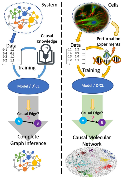
Figure 2.1: Conceptual overview of the proposed learning scheme (left) and its use for large-scale biological experiments (right). We developed a neural architecture for learning causal structures from a combination of empirical data and prior causal knowledge. Learning causal structures from data entails learning a graph G , whose nodes are system variables and whose directed edges encode causal relationships between the variables. Such graphs encode causal – not just correlational – information and their learning remains challenging. In an abstract workflow (left), the proposed learner combines empirical data, obtained from a specific system (with unknown underlying causal structure) with prior causal knowledge, to give an estimate of the unknown causal structure. In an instantiation of the general workflow for biological problems, data is obtained from a specific biological system and causal prior knowledge is derived either from known science or interventional experiments on the system. In the example shown, the problem is high-dimensional since the data matrix spans many different variables whose mutual causal relationships are of interest. The learner combines the sources of information to give an estimate of a graph spanning all nodes of interest, thereby leveraging the limited inputs to generalize to the entire system. During the training phase, the model learns features that help identify causal relationships between variables. During inference, the trained model then decides, for any pair of variables A and B , whether A has a causal influence on A , B on A , or neither.
