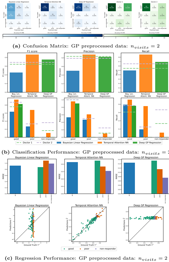
Figure D.3: Entire Population Validation Data: Results of the GP preprocessed dataset with n_{visits} = 2 : (a) Confusion matrix: left algorithms (blue colorbar) and right human ophthalmologists (green colorbar) (b) Classification performance of the Bayesian linear regression (blue), the temporal attention neural network (orange) and the Deep GP (green) are shown. The top row depicts F1 scores, precision and recall values for all patients while the bottom row presents the same metrics per subpopulation. (c) Regression performance for the same models are shown. Top row: The RMSE value of the entire test data is given on the left while class-wise RMSE values are shown on the right of each subplot. Bottom row: Scatter plot presenting predictions against ground truth.
