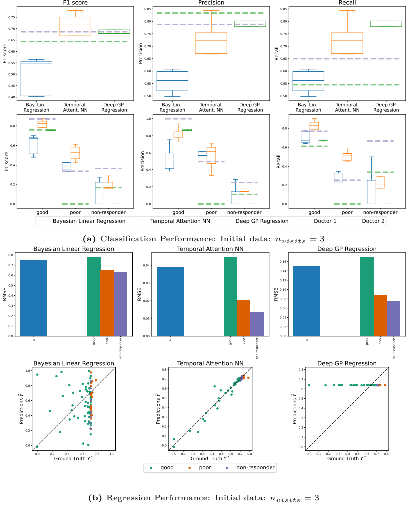
Figure 5.5: Results of the initial dataset with n_{visits} = 3 : (a) Classification performance of the Bayesian linear regression (blue), the temporal attention neural network (orange) and the Deep GP (green) are shown. The top row depicts F1 scores, precision and recall values for all patients while the bottom row presents the same metrics per subpopulation. (b) Regression performance for the same models are shown. Top row: The RMSE value of the entire test data is given on the left while class-wise RMSE values are shown on the right of each subplot. Bottom row: Scatter plot presenting predictions against ground truth.
