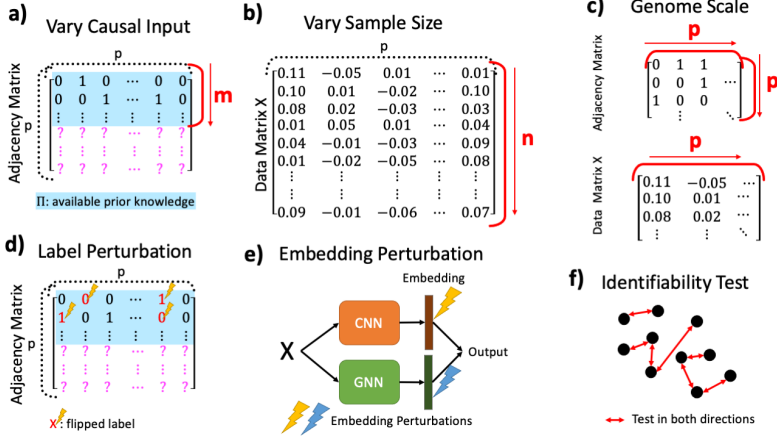
Figure 2.3: Visual illustration of changed configurations in evaluation of yeast gene deletion data (see Text for details): (a) Varying amount of causal input m , (b) Varying sample size n , (c) Scaling to full yeast genome, (d) Label perturbation, (e) Embedding perturbation, (f) Causal direction analysis
