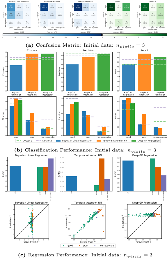
Figure D.4: Entire Population Validation Data: Results of the initial dataset with n_{visits} = 3 : (a) Confusion matrix: left algorithms (blue colorbar) and right human ophthalmologists (green colorbar) (b) Classification performance of the Bayesian linear regression (blue), the temporal attention neural network (orange) and the Deep GP (green) are shown. The top row depicts F1 scores, precision and recall values for all patients while the bottom row presents the same metrics per subpopulation. (c) Regression performance for the same models are shown. Top row: The RMSE value of the entire test data is given on the left while class-wise RMSE values are shown on the right of each subplot. Bottom row: Scatter plot presenting predictions against ground truth.
