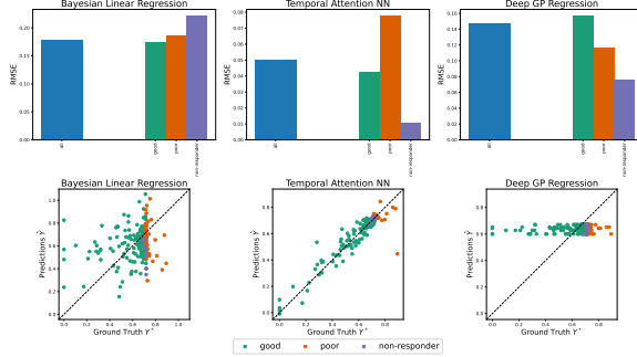
(c) Regression Performance: GP preprocessed data: n_{visits} = 3
