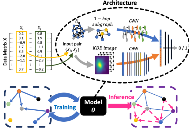
Figure 2.2: Overview of the D 2 CL architecture, training and inference. D 2 CL combines empirical data on a large number of variables with prior causal knowledge to learn causal relationships between variables. For any pair of variables X_i and X_j (corresponding to two columns of the input data matrix), D 2 CL seeks to learn whether X_i has a causal influence on X_j , X_j on X_i , or neither. This is done using a neural architecture with two components: a CNN tower aimed at learning distributional features and a GNN tower that detects structural regularities. For an ordered pair (X_i, X_j) , the CNN tower captures distributional information via a bivariate density estimate that traverses the tower to form an embedding. The GNN tower extracts a 1-hop subgraph from an initial graph G_0 and computes an embedding containing structural information on the neighborhood of the nodes. The CNN and GNN embeddings are then merged through multiple layers which finally output the probability of a directed causal relationship. The input causal information is used to provide a training signal (see text for details). During inference the network generalizes beyond the initial inputs to provide an estimate of the global graph spanning all variables of interest.
