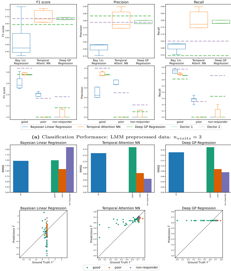
Figure 5.6: Results of the LMM preprocessed dataset with n_{visits} = 3 : (a) Classification performance of the Bayesian linear regression (blue), the temporal attention neural network (orange) and the Deep GP (green) are shown. The top row depicts F1 scores, precision and recall values for all patients while the bottom row presents the same metrics per subpopulation. (b) Regression performance for the same models are shown. Top row: The RMSE value of the entire test data is given on the left while class-wise RMSE values are shown on the right of each subplot. Bottom row: Scatter plot presenting predictions against ground truth.
