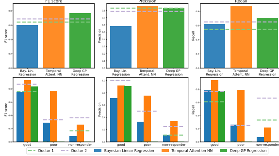
(b) Classification Performance: GP preprocessed data: n_{visits} = 3
