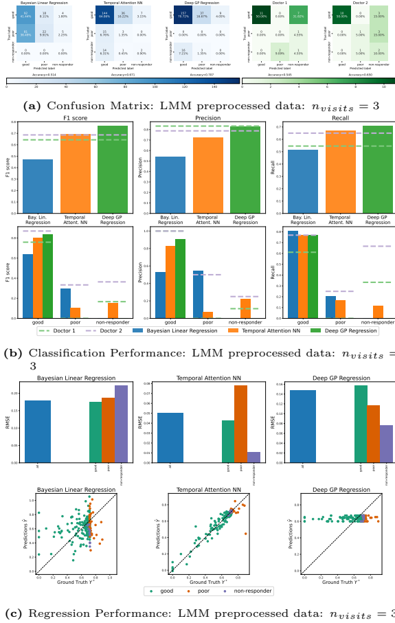
Figure D.5: Entire Population Validation Data: Results of the LMM preprocessed dataset with n_{visits} = 3 : (a) Confusion matrix: left algorithms (blue colorbar) and right human ophthalmologists (green colorbar) (b) Classification performance of the Bayesian linear regression (blue), the temporal attention neural network (orange) and the Deep GP (green) are shown. The top row depicts F1 scores, precision and recall values for all patients while the bottom row presents the same metrics per subpopulation. (c) Regression performance for the same models are shown. Top row: The RMSE value of the entire test data is given on the left while class-wise RMSE values are shown on the right of each subplot. Bottom row: Scatter plot presenting predictions against ground truth.
