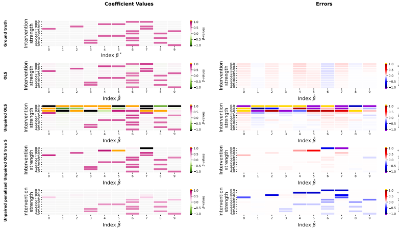
Figure 4.2: Experiment (E1): Intervention strength. (a): Boxplot of RMSE of predicted coefficients \hat{\beta} (left) and predicted outcomes Y (right) for OLS (blue), Unpaired OLS (orange), Unpaired OLS using solely non-coefficients (green) and our proposed penalized covariance adjusted estimator, Unpaired penalized, (red). (b): Heatmap of ground truth and predicted \beta -coefficients (left), error between predictions and ground truth values (right), lighter colors indicate smaller errors. Predicted \beta -values falling outside the range of [-1, 1] are represented in black and orange, while errors exceeding [-1, 1] are emphasized using purple and gold.
