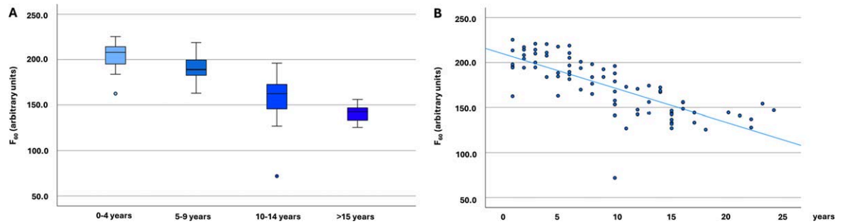
Fig. 1. \alpha -Synuclein seeding in Parkinson's disease cohorts ( n = 79 ). A) \alpha -Synuclein seeding in Parkinson's disease cohorts with different disease duration ( n = 79 ). The boxplots indicate the median (range) Thioflavin T signal intensity after 60 hours (in arbitrary units) of the four different Parkinson's disease duration groups. B) Scatter diagram showing the correlation of \alpha -synuclein seeding (Thioflavin T signal intensity after 60 hours) and disease duration in all analyzed individuals with Parkinson's disease ( n = 79 ). F 60 , Thioflavin T signal intensity after 60 hours; PD, Parkinson's disease.
