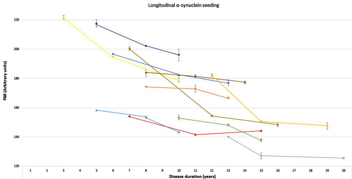
Fig. 2. Longitudinal \alpha -synuclein seeding of individuals with Parkinson's disease. Presentation of longitudinal values of the \alpha -synuclein seed amplification assay in n = 11 individuals with Parkinson's disease at three timepoints. \alpha -Synucleins seeding is displayed as Thioflavin T signal intensity after 60 hours (F60). Each colored line represents longitudinal values of one individual with Parkinson's disease (mean of both replicates, error bars indicate the standard deviation of both replicates). F60, Thioflavin T signal intensity after 60 hours.
