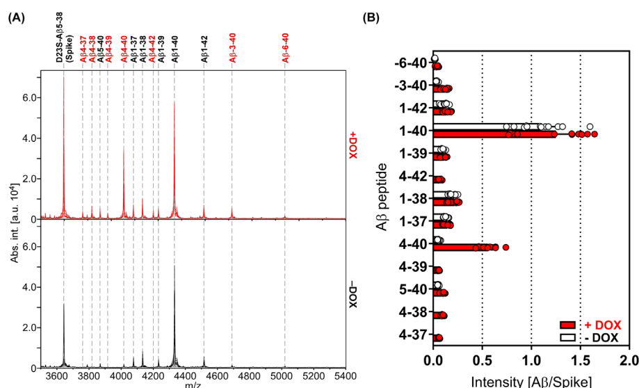
FIGURE 3 MALDI-TOF mass spectra of Aβ peptides immunoprecipitated from HEK293-APP695wt/ADAMTS4 cells. (A) Aliquots of conditioned cell culture media of HEK293-APP695wt/ADAMTS4 cells with (+DOX) and without (–DOX) induction of ADAMTS4 expression were subjected to immunoprecipitation with 6E10-coupled magnetic beads and analysed by MALDI-TOF-MS. The artificial model peptide Aβ5–38(D23S) was added as a spike for normalisation. An overlay of 12 linear mode mass spectra per condition is shown. Black and red traces correspond to samples without (–DOX) and with (+DOX) induction of ADAMTS4 expression, respectively. The annotation of Aβ signals was based on monoisotopic masses derived from reflector mode mass spectra (see Table S2A,B). (B) Quantitative comparison of the Aβ signals shown in (A). The ratio of the signal intensities of the Aβ peptide of interest divided by the signal intensity of the Aβ5–38(D23S) peptide used for normalisation was calculated. Significant differences in normalised signal intensities after induction of ADAMTS4 expression were observed for Aβ3–40, Aβ6–40, Aβ4–40 and Aβ5–40 peptides (mean \pm SD, multiple t tests). Note that signals for Aβ4–37, Aβ4–38, Aβ4–39 and Aβ4–42 were undetectable in noninduced cells and thus not included in the statistical analysis. The 12 mass spectra per condition were obtained from three individual IPs, two MALDI preparations per IP, and two measurements per preparation.
