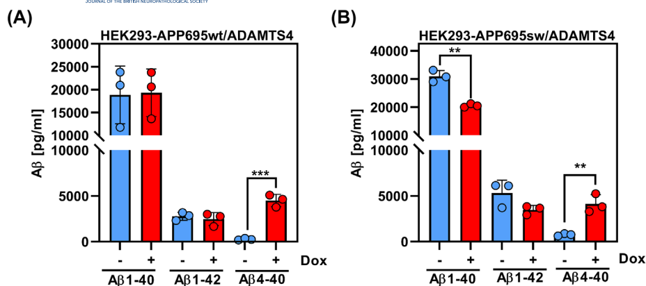
FIGURE 2 ELISA measurements of Aβ1-x and Aβ4-x peptides in conditioned culture supernatants of HEK293 cells with inducible overexpression of ADAMTS4. (A) In HEK293-APP695wt/ADAMTS4 cells, Aβ1-40 and Aβ1-42 levels were unchanged while Aβ4-40 levels were significantly increased after ADAMTS4 induction as compared with noninduced control cells. (B) Similarly, in HEK293-APP695sw/ADAMTS4 cells, induction of ADAMTS4 expression resulted in significantly increased Aβ4-40 levels, while Aβ1-40 levels were reduced. Three independent biological experiments for each cell line were performed ( n = 3 ). DOX—doxycycline, ** p < 0.01 , *** p < 0.001 , mean \pm SD, unpaired t test.
