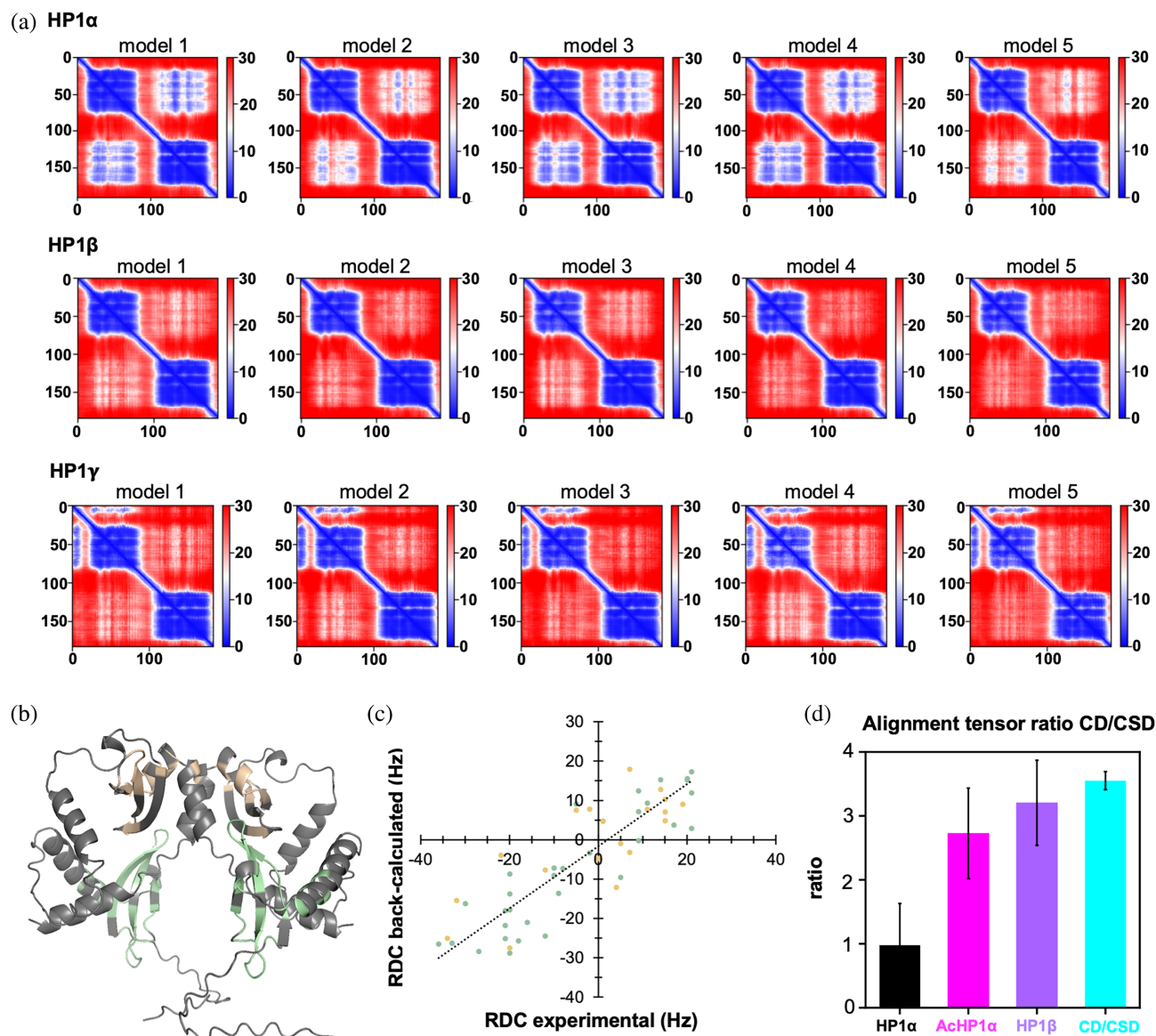
FIGURE 2 HP1α CD/CSD arrangement differs from HP1β and HP1γ. (a) Aligned errors for five model structures predicted by AlphaFold2 for HP1α (top), HP1β (middle), and HP1γ (bottom). The color at position (x, y) indicates AlphaFold2's expected position error at residue x, when the predicted and true structures are aligned on residue y. (b) HP1α dimer model predicted by the multimer model of AlphaFold2 (Jumper et al., 2021; Mirdita et al., 2022); residues highlighted in green (CD) and orange (CSD) were used for RDC analysis (see Figure 2c). (c) Correlation between experimental ^1\text{H} - ^{15}\text{N} RDCs and RDCs back-calculated from the AlphaFold2-predicted 3D structure of the HP1α dimer shown in (b). (d) Ratios of the RDC-derived alignment tensor magnitudes \text{Da}(\text{HN}) between the CD and the CSD, that is, \text{Da}(\text{HN})^{\text{CD}}/\text{Da}(\text{HN})^{\text{CSD}} , in full-length HP1α (black), AcHP1α (magenta), and HP1β (violet). For comparison, the CSD/CD ratio of alignment magnitudes predicted by PALES for the individual CSD and CD domains of HP1α and HP1β are shown in cyan. Error bars represent std. CD, chromodomain; CSD, chromoshadow domain; RDC, residual dipolar coupling.
