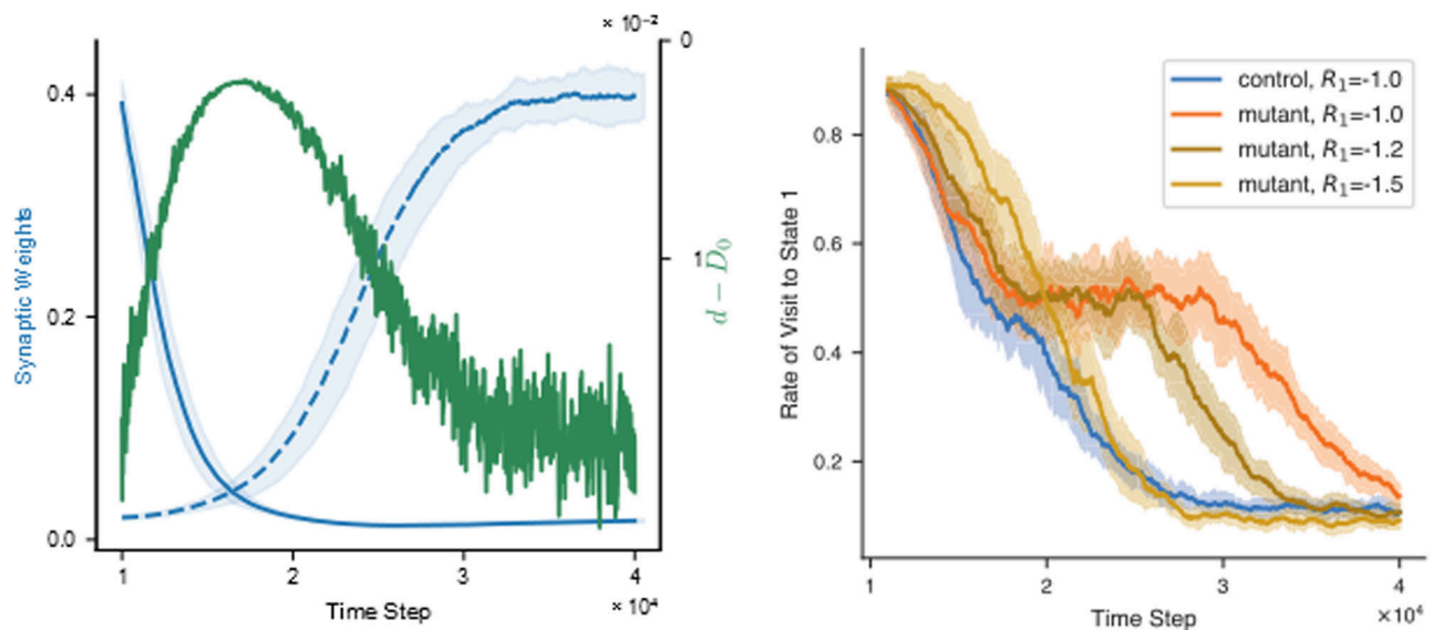
Fig. 5 | (left) Increased D-serine levels during reverse learning. The blue lines are the evolution of the two synaptic weights during reverse learning of normal mice (same lines of Fig. 4, bottom graph, second phase). The D-serine concentration relative to its maximum value D_0 is superposed (green line). The scale for d - D_0 is of course different from that of the synaptic weights, and it is drawn on the right axis. The D-serine levels increase during reverse learning and they return to the basal value when the switching is completed. This prediction suggests that the astrocytic regulation of D-serine has the specific function of enhancing plasticity response to changes in the external
