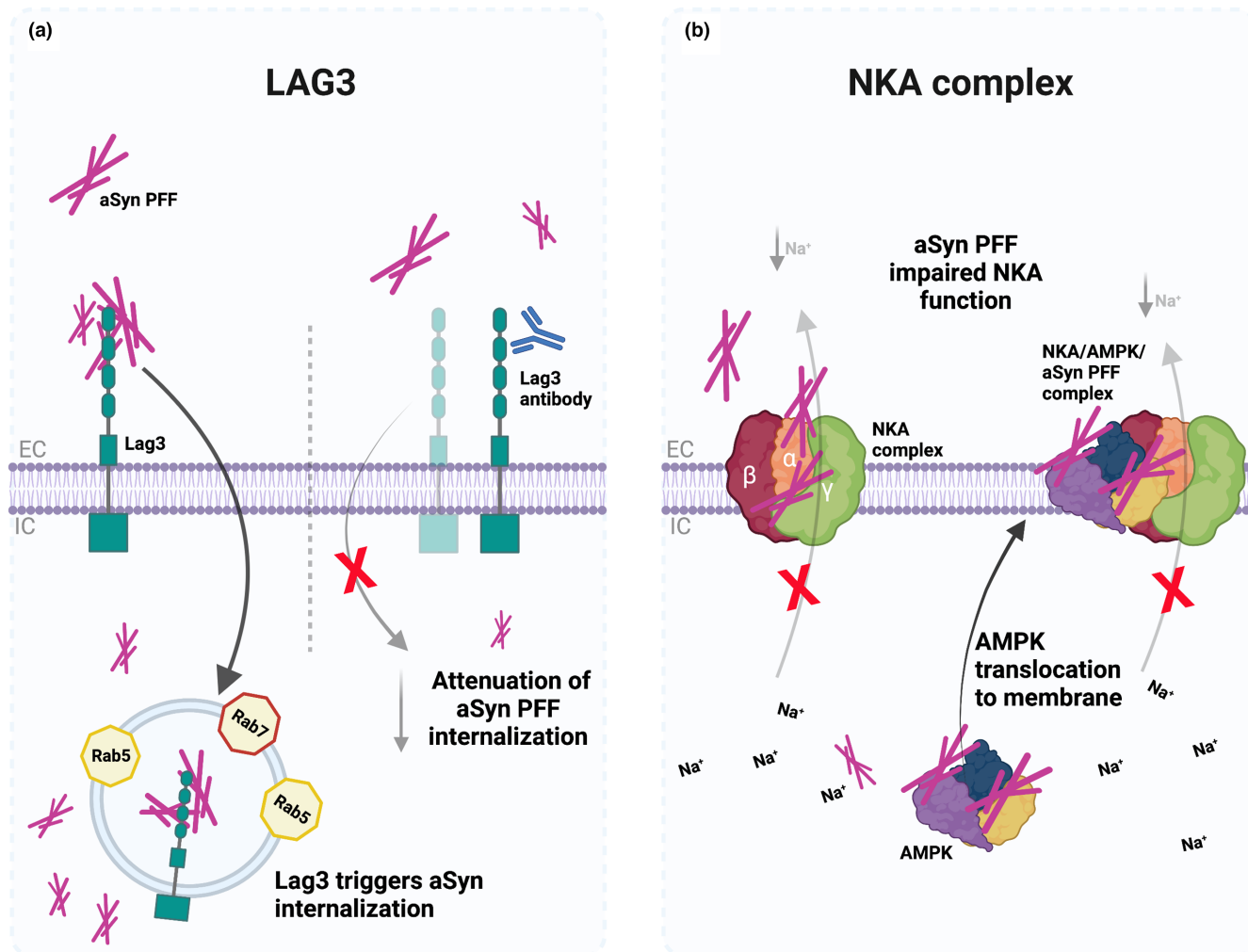
FIGURE 4 Lymphocyte-activation gene 3 (Lag3) and Na + /K + -ATPase (NKA) are involved in the internalization of alpha-synuclein (aSyn) preformed fibers (PFF). (a) Lag3 can directly interact with aSyn PFF, promoting their internalization across the cell membrane. Rab5 and Rab7 participate in this process. The absence of Lag3, or the use of Lag3 antibodies, attenuates the propagation of aSyn PFF. (b) The presence of aSyn aggregates impairs NKA function by interacting with the extracellular segments of \alpha 3-NKA. Another possibility is that the interaction of aSyn PFF with AMPK may contribute to the translocation of AMPK to the cell membrane and promote interaction with NKA. Thus, NKA function may also be impaired by the formation of the NKA/AMPK/PFF complex. Created with BioRender.com.
