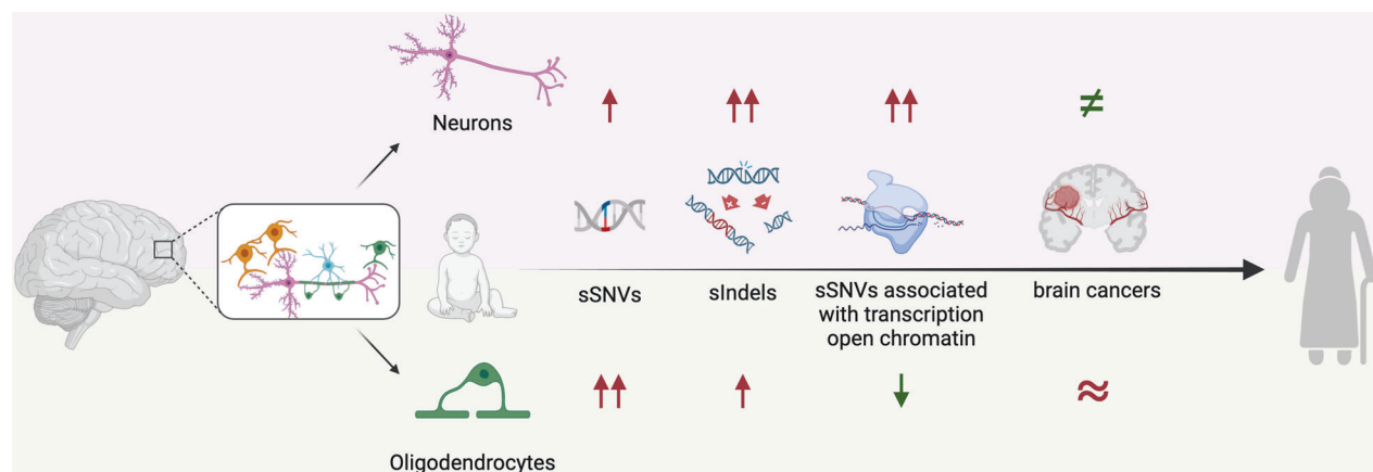
Fig. 1 Schematic representation of findings by Ganz et al. 1 highlighting differences in somatic mutations between neurons and oligodendrocytes. sSNVs: somatic single nucleotide variants; sIndels: somatic insertions and deletions. Created with BioRender.com
