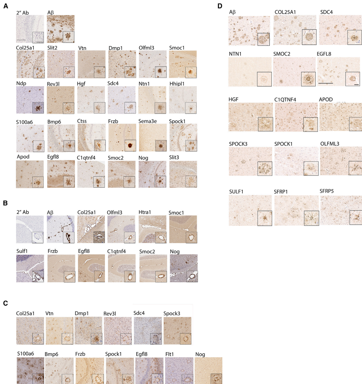
Figure 5. M42+ DEPs colocalize with amyloid pathology
