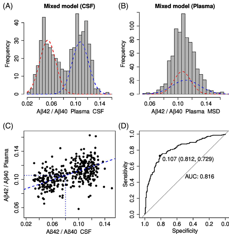
FIGURE 2 Mixture modeling analysis of the A\beta_{42}/A\beta_{40} ratio in plasma and CSF. Mixture modeling analysis revealed a typical bimodal distribution for CSF (A) but not A\beta_{42}/A\beta_{40} in IP eluates from plasma (B). To determine the A\beta_{42}/A\beta_{40} cutoff value in plasma, A\beta_{42}/A\beta_{40} values in CSF were correlated with the corresponding A\beta_{42}/A\beta_{40} values in plasma via a linear regression model (C). The intersection of the dashed blue lines indicates the 0.106 cutoff value for plasma A\beta_{42}/A\beta_{40} . In (D), the receiver-operating characteristic (ROC) curve was plotted with an area under the curve (AUC) of 0.81 for A\beta_{42}/A\beta_{40} to predict amyloid positivity based on A\beta_{42}/A\beta_{40} classification in CSF. A\beta_{42}/A\beta_{40} , amyloid beta X-42/amyloid beta X-40; CSF, cerebrospinal fluid.
