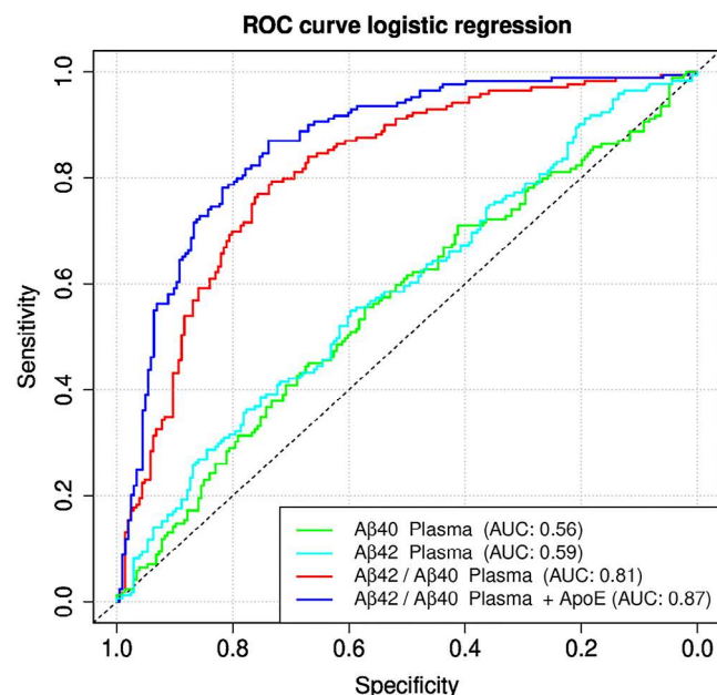
FIGURE 3 Receiver-operating characteristic curves for the A \beta 40 and A \beta 42, A \beta 42/A \beta 40 ratio, and A \beta 42/A \beta 40 ratio + APOE \epsilon 4 carriage. For the plasma A \beta 42/A \beta 40 ratio, we calculated a receiver-operating characteristic (ROC) curve comparing amyloid-positive against amyloid-negative cases with an area under the curve (AUC) of 0.81. However, when stratified by APOE \epsilon 4 positivity, the AUC rose as high as 0.87, with a 0.73 corresponding specificity and 0.87 sensitivity. Significantly lower AUCs were found for A \beta 40 at 0.56 and for A \beta 42 plasma at 0.59. A \beta 40, amyloid beta X-40; A \beta 42, amyloid beta X-42; A \beta 42/A \beta 40, amyloid beta X-42/amyloid beta X-40 ratio; APOE \epsilon 4, apolipoprotein E \epsilon 4.
