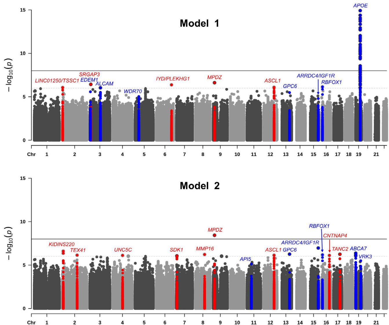
FIGURE 1 Manhattan plots showing negative log 10 -transformed p-values from the single-variant meta-analysis adjusted for age, sex, and population stratification (Model 1) and age, sex, population stratification, and APOE (Model 2). The solid black horizontal line represents a genome-wide significance threshold of p = 5 \times 10^{-8} , and the dotted line represents a suggestive threshold of p = 5 \times 10^{-6} . All novel loci significant at p < 9 \times 10^{-7} are shown in red, and all previously reported loci significant at p < 9 \times 10^{-6} are shown in blue. The y-axis has been truncated, the lowest p value on chromosome 19 is 3.11 \times 10^{-65} .
