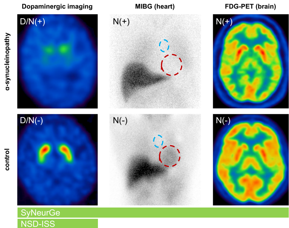
Fig. 1 Schematic overview on imaging biomarkers of the dopaminergic system and neurodegeneration in PD and DLB as proposed by SyNeurGe and NSD-ISS
