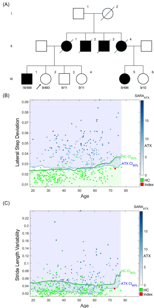
FIG. 1. Pedigree of the German family with SCA27B and quantitative gait analysis. (A) Pedigree of the German family with spinocerebellar ataxia 27B (SCA27B). The allele sizes, expressed as numbers of GAA repeat units, are provided for the family members who underwent genotyping of the FGF14 repeat locus. Squares represent male family members and circles female family members. Solid black shapes indicate affected persons. Slashed symbols indicate deceased persons. The pedigree has been abbreviated and family members randomly rearranged to preserve privacy. The subject of this study is indicated by a black arrow. Comparison of (B) lateral step deviation and (C) stride length variability by quantitative gait analysis using APDM wearable sensors between the index subject (red dot), healthy controls (HC, green), and patients with degenerative cerebellar ataxia (ATX, blue), according to their age at time of assessment. The green line indicates the upper bound of the 90% confidence interval around the average gait performance of healthy controls. The blue line indicates the lower bound of the 90% confidence interval around the average gait performance of ataxic patients. The color of the data points for the ataxic individuals is a function of the severity of ataxia as measured by the Scale for the Assessment and Rating of Ataxia (SARA) score, with dark blue indicating more severe ataxia (a hue scale is shown on the right y-axis). [Color figure can be viewed at wileyonlinelibrary.com ]
