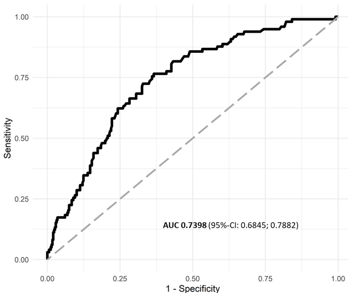
Figure 4. ROC analysis for ventilation time in predicting POD. Note. ROC = receiver operating characteristics; POD = postoperative delirium; AUC = area under the curve; CI = confidence interval. AUC is reported below the ROC curve.
