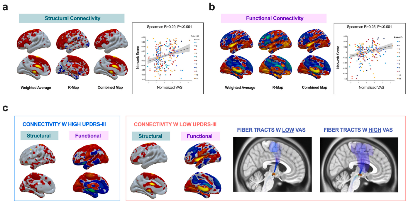
Fig. 2. Patient subjective ratings correlate with beneficial brain network connectivity. (a,b) Images depicting structural and functional connectivity maps determined through a weighted average (first column), correlation analysis with VAS (R maps, second column), and a combination of these maps (third column) associated with VAS ratings. Graphs illustrating the correlation of VAS with connectivity; a leave-one-cohort-out approach was used to predict VAS ratings of each patient through the combined map. (c) Images illustrating structural and functional connectivity maps (combined maps) of two representative cases with a high or low UPDRS-III score (Med On/Stim On), respectively. Right panel: Topography of the white matter tracts from the case with the lowest UPDRS-III score associated with the highest and lowest VAS values obtained during the study visit.
