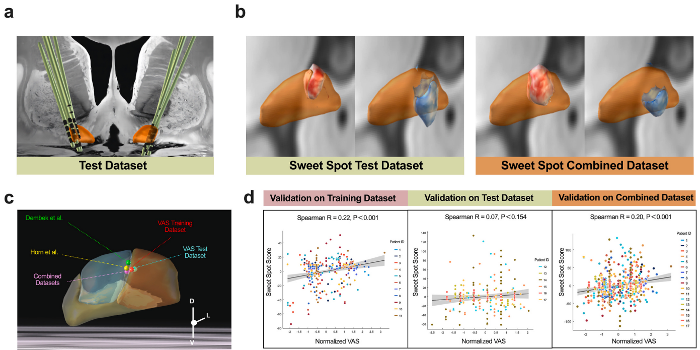
Fig. 3. Validation of VAS based sweet and sour spots in a separate dataset. (a) Electrode reconstructions from individual patients in the test dataset (n = 6). (b) Images displaying the locations of sweet and sour spots identified in the test dataset (left), as well as those identified when combining data sets (right). (c) Illustration comparing the center of mass of sweet spots by MNI coordinates in each dataset with previously published sweet spots [37,40]. (d) Graphs demonstrating the predictive accuracy of VAS sweet spots between training and test dataset through cross-validation. Validation on training dataset (left) perform better predictive capability than validation on test dataset (middle). Combined dataset prediction further reveals the robustness of VAS sweet spots predictive capability by leave-one-cohort-out fashion (right).
