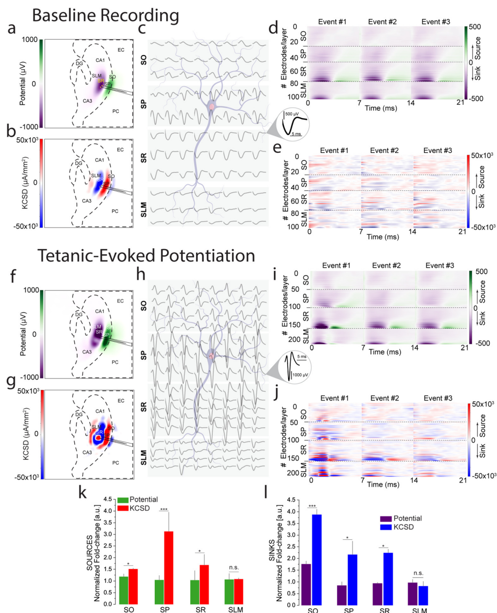
FIG. 5. Mesoscale mapping of network synaptic activity and connectivity dynamics. (a), (b), (f), and (g) Bidimensional maps showing potential-based and kernel current source density (KCSD) representations of synaptic activity in the CA1–CA3 network under baseline and post-tetanic stimulation conditions. (c) and (h) Extracellular potential signatures across different hippocampal layers, illustrating network-level synaptic dynamics and connectivity changes from baseline to tetanic-evoked potentiation. (d), (e), (i), and (j) Time-resolved synaptic activity maps, with the x-axis representing the timing of evoked events and the y-axis corresponding to firing electrodes within each layer. These maps provide a detailed view of sinks (associated with incoming EPSPs) and sources (related to synchronous neuronal firing). (k) and (l) Comparison of quantified potential sources and sinks against those identified in the KCSD maps, highlighting the KCSD analysis's superior precision in localizing synaptic events. This approach enhances our understanding of synaptic transmission and network dynamics in response to LTP, revealing intricate differences in sink and source values both at baseline and post-tetanic conditions.
