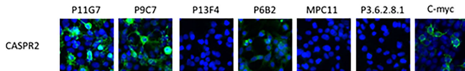
Fig. 3 Identification of anti-Caspr2 antibody target domains. A Caspr2 mutant constructs. The extracellular portion of Caspr2 has 8 domains. The mutant constructs each missing one of the domains were previously generated [25]. Deletions are indicated by the respective amino acid positions (Δaa-aa). The Disc iso construct contains only the discoidin domain. B HEK293T cells were transfected with one of the Caspr2 mutant constructs for 48 h and incubated with each anti-Caspr2 antibody using live staining. P11G7 and P9C7 bind to all mutant constructs except the one missing the discoidin domain. P6B2 and P13F4 do not bind to any of the constructs. Isotype controls showed no binding to any construct. C P11G7 and P9C7 bind to the discoidin domain only construct. P13F4 and P6B2 do not bind to the discoidin domain only construct. D P11G7, P9C7, bind to Caspr2 transfected HEK293T cells. P6B2, P13F4 and the isotype controls do not.
