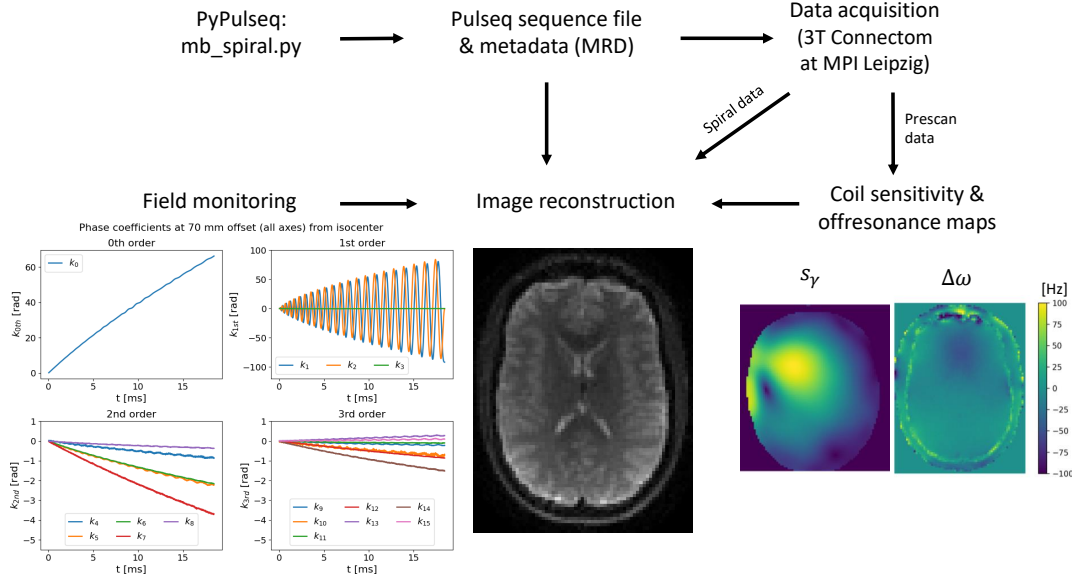
Figure 4.1: Spiral sequence development and image reconstruction pipeline [112]. The spiral sequence was designed using PyPulseseq and Pulseseq. The sequence includes a dual-echo gradient echo (GRE) prescan for coil sensitivity calibration and mapping of static off-resonance. Image reconstruction with an expanded encoding model was implemented in the PowerGrid toolbox using k -space phase coefficients of up to third spatial order. An example set of phase coefficients measured with a field camera (Skopec) is shown on the left.
