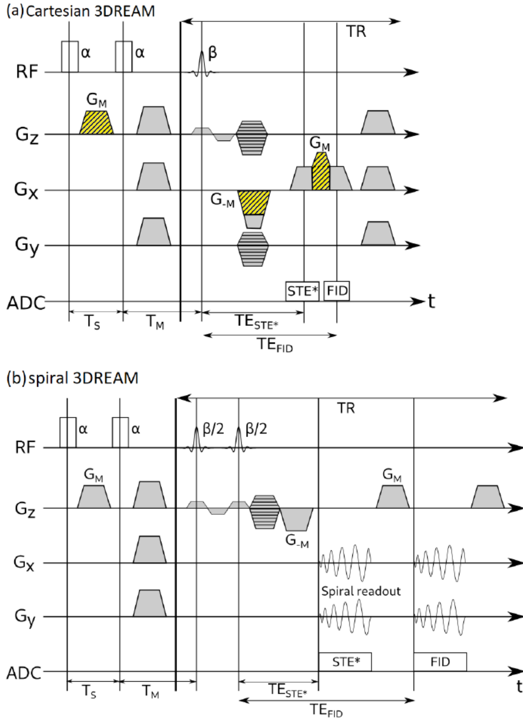
Figure A7: (a) The sequence diagram of the modified Cartesian 3DREAM with an additional spoiler moment (highlighted in yellow) between the STE* and FID readouts to better separate the signals in k -space. (b) The sequence diagram of the spiral 3DREAM sequence (Figure 1) with signal separation gradients in slice direction.
