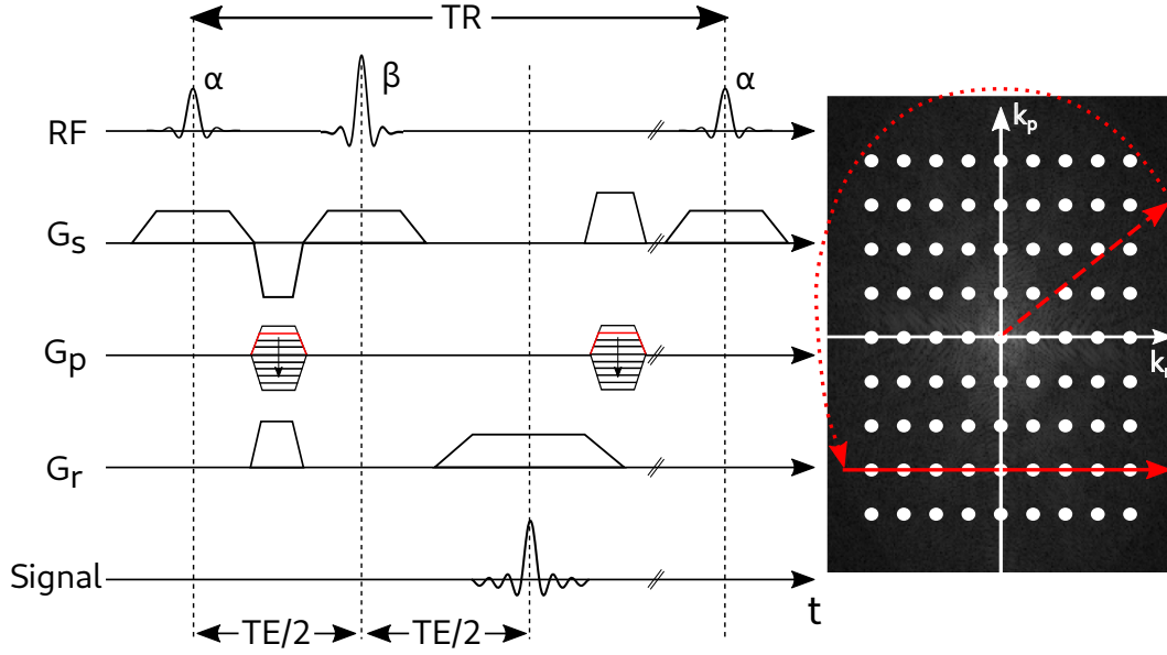
Figure 2.3: Spin echo sequence timing diagram with RF, gradient and signal axes. The acquisition of one k -space line selected by the phase encoding gradient is illustrated on the right. After the refocusing pulse, the k -space position is flipped around the k -space center.
