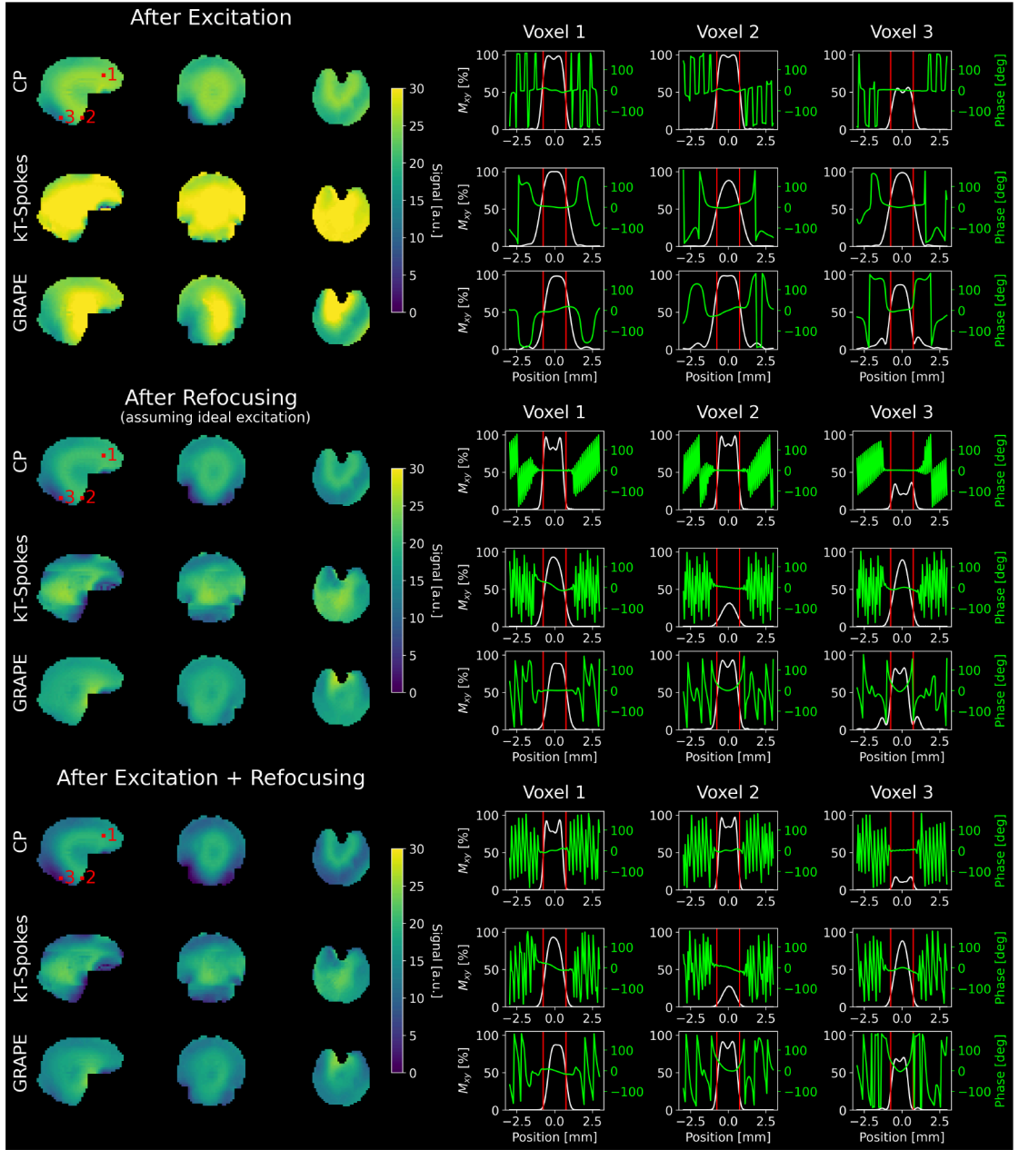
Figure 6.2: Left: Simulated signal of CP, kT-Spokes and GRAPE pulses after excitation, refocusing (assuming ideal excitation) and successive application of both pulses. The displayed signal level per voxel is the integral of the simulated transverse magnetization in slice direction. Mean and standard deviation of the signal over the whole brain after excitation were: CP: 21.8 \pm 3.3 , Spokes: 28.6 \pm 2.6 , GRAPE: 23.9 \pm 4.3 . After refocusing: CP: 17.1 \pm 3.9 , Spokes: 17.4 \pm 4.0 , GRAPE: 18.0 \pm 2.3 . After both pulses: CP: 13.5 \pm 4.6 , Spokes: 15.4 \pm 4.0 , GRAPE: 15.3 \pm 2.9 . Right: Simulated transverse magnetization of CP, kT-Spokes and GRAPE pulses along the slice direction at three distinct positions. The positions are marked in the sagittal slice of the CP signal maps. The Bloch simulations were done along a 6 mm line in slice direction. The red vertical lines show the target slice thickness of 1.5 mm. The magnitude of the transverse magnetization in percent of the initial magnetization is shown in white and the phase is shown in green.
