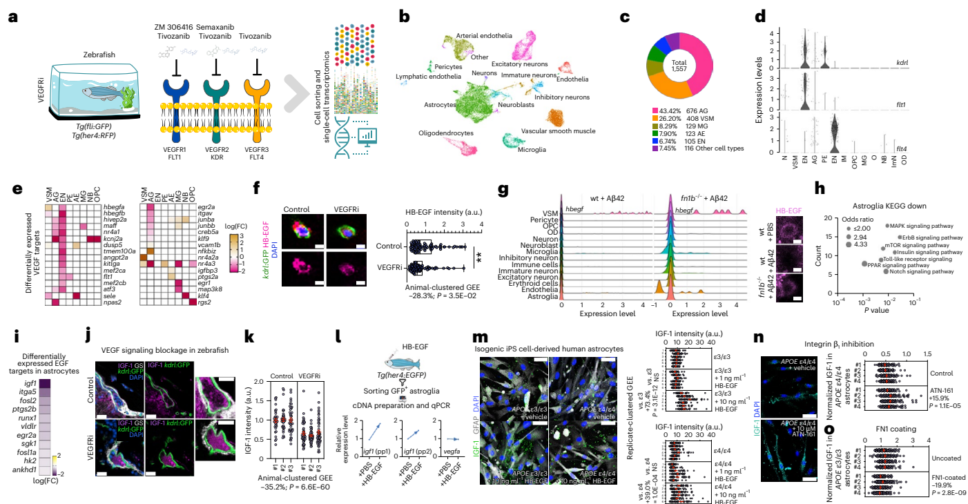
Fig. 6 | VEGF signaling is required for HB-EGF expression and subsequent IGF-1 induction. a , Schematic of the VEGFRi study and subsequent single-cell transcriptomics in the double reporter zebrafish line Tg(fli1a:EGFP) 61 and Tg(her4:RFP) 62 , marking endothelial cells and astrocytes, respectively. b , UMAP of the identified cell types. c , Distribution of DEGs among cell types. d , Violin plots showing the expression of the VEGFRs kdr1 , flt1 and flt4 in cell types. e , Heat map of differential expression of selected VEGF target genes in major cell types from b and c . AE, arterial endothelia; VSM, vascular smooth muscle; N, neuron; O, other. f , Immunostaining for HB-EGF and kdr :GFP with DAPI counterstain in control and VEGFRi zebrafish brains showing single vasculature (left), along with a quantification graph for HB-EGF (right). VEGFRi reduces HB-EGF levels. Each data point represents one gliovascular contact point. Measurements were obtained from n = 4 independent animals per group. Multiple contact points were analyzed per animal, and statistical inference was performed at the animal level using GEEs (two-sided). Violin plots show the data distribution; the center line indicates the median; the box represents the interquartile range (25th–75th percentile); whiskers extend to the minimum and maximum values; points represent individual observations. g , Left: ridge plot for hbegf expression in control + Aβ42 and fn1b -/- + Aβ42 zebrafish brains indicating upregulation in endothelia. Right: immunostaining for HB-EGF. h , Multivariable graph for downregulated pathways in astrocytes, showing enrichment of MAPK, ErbB, mTOR and insulin signaling pathways. PPAR, peroxisome proliferator-activated receptor. i , Heat map showing differential expression of selected EGF target genes in astrocytes after VEGFRi. j , Immunofluorescence staining for IGF-1, GS
