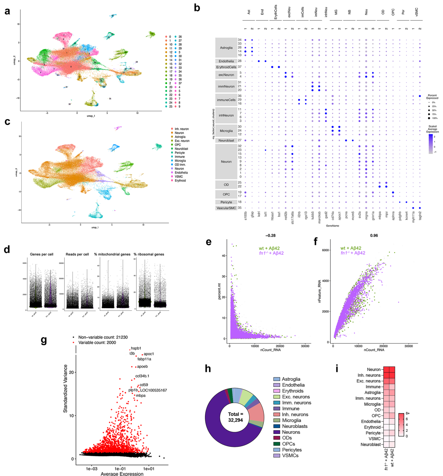
Extended Data Fig. 6 | Single cell transcriptomics in fn1b homozygous knockout animals after A \beta 42. a , UMAP for 38 clusters. b , Dot plot for cell type markers. c , UMAP with cell types color-coded. d , Violin plots for genes per cell, reads per cell, percent mitochondrial gene expression and percent ribosomal gene expression. e , Distribution graphs for percent mitochondrial gene expression against reads per cell in wt + A \beta 42 and fn1b -/- + A \beta 42 samples.
