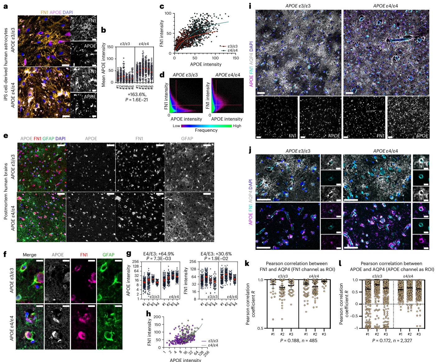
Fig. 3 | FN1 colocalizes with APOE4. a , Immunofluorescence staining for FN1 and APOE with DAPI counterstain (blue) in APOE \epsilon 3/\epsilon 3 and APOE \epsilon 4/\epsilon 4 isogenic iPS cell-derived human astrocytes. Single channels in white show FN1 and APOE. b , Quantification of APOE protein intensity in extracellular locations. Each data point represents one independent biological replicate (well). n = 6 independent biological replicates. Data are presented as mean \pm s.e.m. Statistical test: replicate-clustered GEE (two-sided). c , Correlation graph for APOE and FN1 intensities in APOE \epsilon 3/\epsilon 3 and APOE \epsilon 4/\epsilon 4 astrocytes. d , Colocalization histogram for APOE and FN1. The upper right quadrant shows colocalization, which is enriched in APOE \epsilon 4/\epsilon 4 . e , Immunofluorescence staining for FN1, APOE and GFAP with DAPI counterstain in APOE \epsilon 3/\epsilon 3 and APOE \epsilon 4/\epsilon 4 postmortem human brain samples from AD cases. Single channels in white show FN1, APOE and GFAP individually. f , High-magnification views from a smaller region of the brains shown in e , illustrating colocalization of APOE and FN1 at the GFAP-enwrapped BBB predominantly in the APOE \epsilon 4/\epsilon 4 case. g , Quantification of APOE and FN1 intensities in human brains. Measurements were obtained from n = 4 APOE \epsilon 3/\epsilon 3 AD donors and n = 4 APOE \epsilon 4/\epsilon 4 AD donors. Multiple ROIs were analyzed per donor, and statistical inference was performed at the donor level using GEEs (two-sided). Data are presented as mean \pm s.e.m. h , Correlation graph for APOE and FN1 intensities in APOE \epsilon 3/\epsilon 3 and APOE \epsilon 4/\epsilon 4 AD cases. i , Representative confocal images of cortical tissue from APOE \epsilon 3/\epsilon 3 and APOE \epsilon 4/\epsilon 4 individuals,
