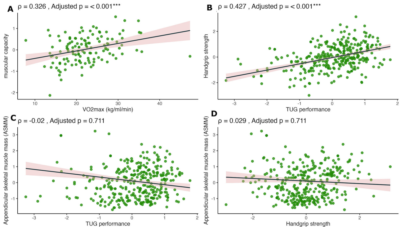
Fig. 1 | Bivariate associations between physical fitness outcomes. A shows \text{VO}_2\text{max} (aerobic capacity, in ml/min/kg) and muscular capacity (z-composite: timed-up-and-go (TUG) test performance, maximal handgrip strength, and appendicular skeletal muscle mass [ASMM]). B–D show the muscular capacity
